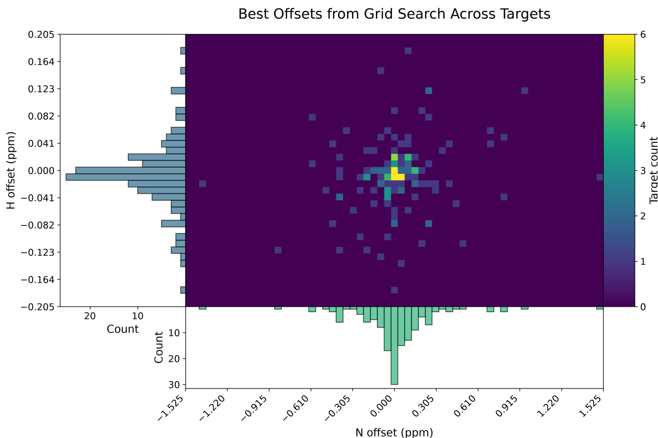
SI Fig. S17. Ideal ^1\text{H}/^{15}\text{N} chemical-shift offset grid for the n = 145 buffer-similar systems in CSP_UBQ_ph0.5_temp5C.csv. For each target, a grid search selects the H/N referencing offsets that maximize aligned HN peak counts under the pipeline CSP criterion; the heatmap aggregates those optimal (\Delta\delta_{\text{N}}, \Delta\delta_{\text{H}}) pairs (color = number of targets). Marginal histograms show the one-dimensional distributions of best H (left) and N (bottom) offsets. Both are peaked near zero, indicating that most apo/holo pairs require only small referencing corrections.
