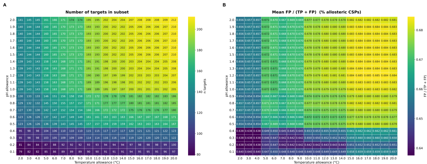
SI Fig. S16. Buffer pH/temperature threshold sweep
