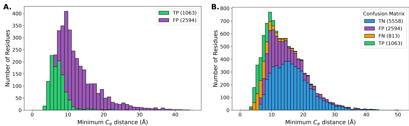
SI Fig. S8. Confusion Matrix Histograms for targets with dissimilar apo/olo experimental conditions ( n = 108 )
