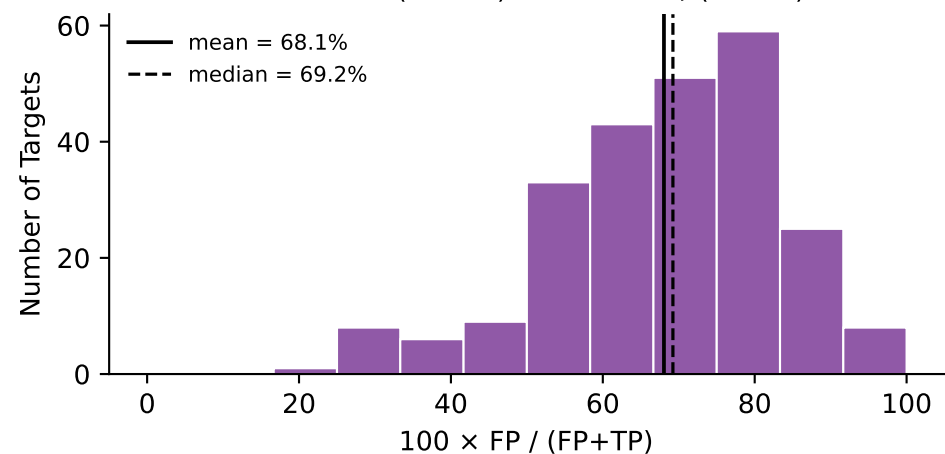
Full CSPdb (n=243) — 100 \times \text{FP} / (\text{TP} + \text{FP})
