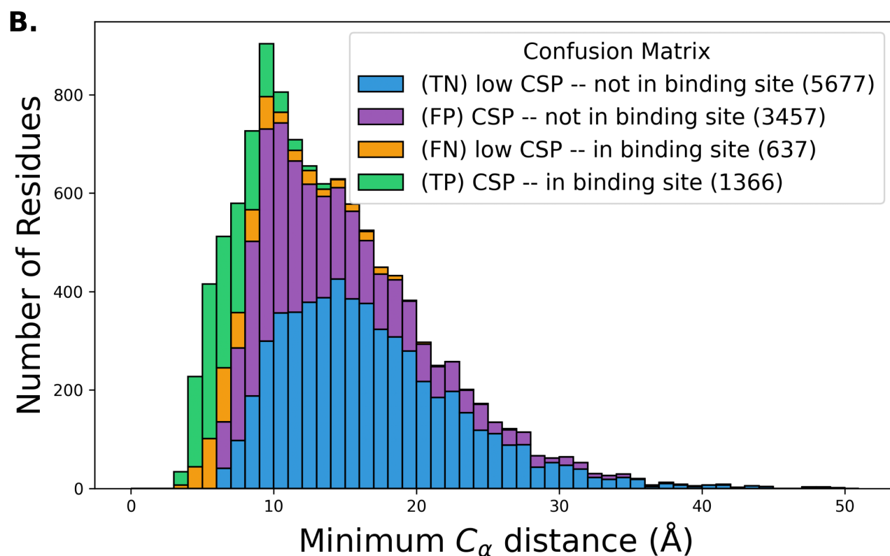
SI Fig. S11. CA-inclusive CSP confusion histograms for the n = 121 buffer-similar systems from CSP_UBQ_ph0.5_temp5C.csv with CA row coverage > 50\% . These results are very similar to CSPs calculated using SI Equation S1. 71.7% of CSPs using SI Equation S2 are distant from the binding site compared to 69.4% using SI Equation S1.
