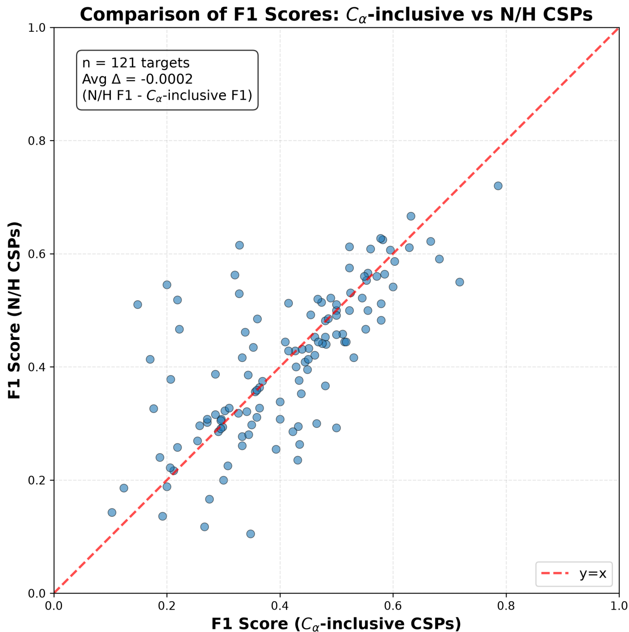
SI Fig. S12. F1 scores for CA-inclusive vs exclusive CSPs ( n = 121 buffer-similar systems from CSP_UBQ_ph0.5_temp5C.csv with CA row coverage > 50\% ). F1 scores on the y axis use SI Equation S1 (combined HN); F1 scores on the x axis use SI Equation S2 (combined HN+ C_\alpha ). The F1 scores here demonstrate that per-target there are very few differences in the distribution of CSPs distant from the binding site across the n = 121 subset of targets with CA CSPs and similar experimental conditions.
