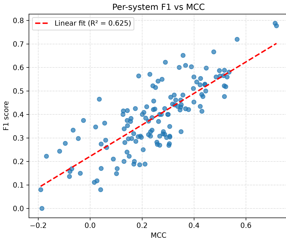
SI Fig. S26. F1 vs MCC across the n = 135 buffer-similar systems in CSP_UBQ_ph0.5_temp5C.csv with pipeline outputs. This figure reveals a strong correlation between F1 and MCC measures against the n = 135 subset. F1 and MCC are both useful metrics to gauge at a glance the extent of distal CSPs are present in the receptor-ligand system 11 .
