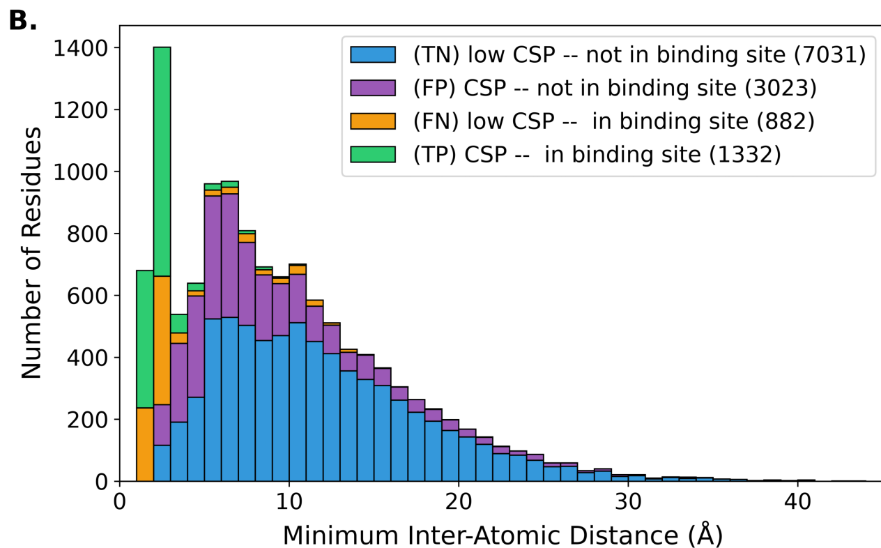
SI Fig. S14. Confusion histograms by closest interchain any-atom distance ( n = 135 buffer-similar systems from CSP_UBQ_ph0.5_temp5C.csv with pipeline outputs).
