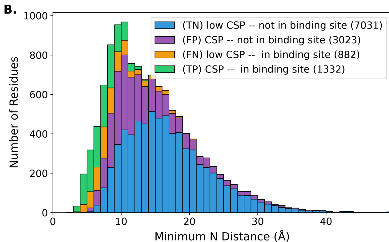
SI Fig. S13. Confusion histograms by closest interchain N–N distance ( n = 135 buffer-similar systems from CSP_UBQ_ph0.5_temp5C.csv with pipeline outputs).
