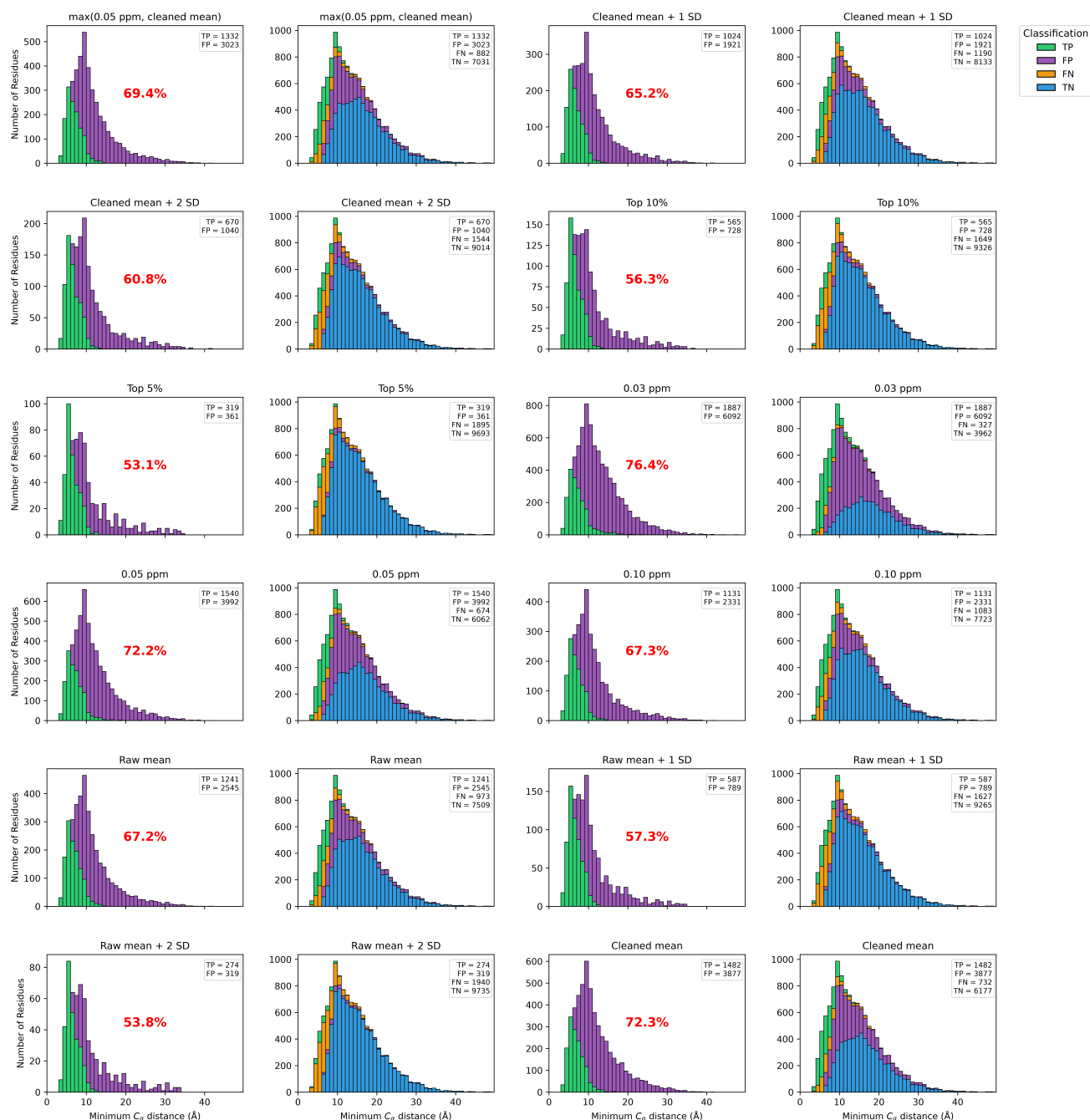
SI Fig. S24. Figure 3-style C_\alpha -distance histograms under alternate HN CSP significance thresholds ( n = 135 buffer-similar systems from CSP_UBQ_ph0.5_temp5C.csv with pipeline outputs). Each column is a 3a (TP/FP among significant CSPs) | 3b (full confusion) pair. Thresholds (left to right, then continuing as labeled on the figure): primary max(cleaned mean, 0.05 ppm) after iterative outlier removal; cleaned mean +1 SD and +2 SD; top 10% and top 5% of HN CSP values; fixed cutoffs 0.03 , 0.05 , and 0.10 ppm ; raw mean , raw mean +1 SD, and raw mean +2 SD (no outlier removal); and cleaned mean without the 0.05 ppm floor. This figure reveals our results are relatively stable if we use other reasonable thresholds of what is considered a significant CSP. Some thresholds from this figure we determine are too high (e.g. Raw mean + 1 SD, Raw mean + 2 SD, Top 10%, Top 5%) which results in less distal CSPs than is expected from the other thresholding approaches.
