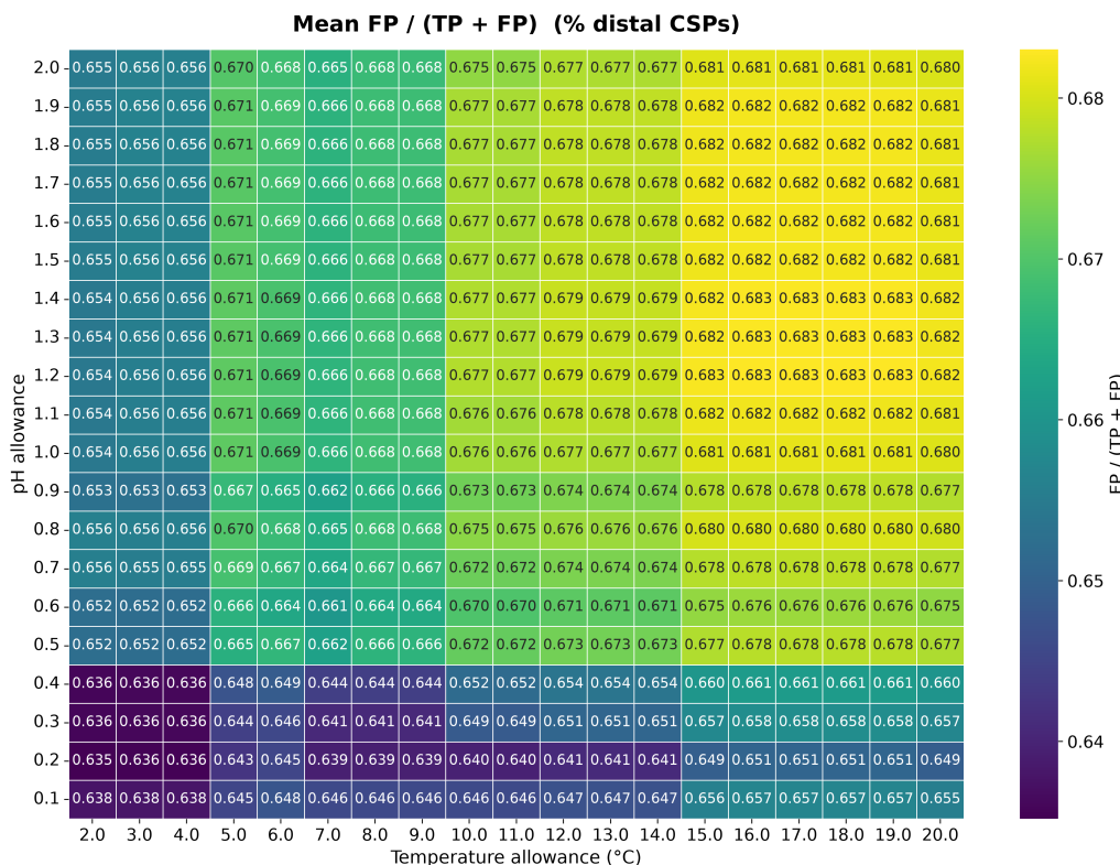
SI Fig. S20. Buffer pH/temperature threshold sweep. A. Number of apo/holo pairs retained as |\Delta\text{pH}| and |\Delta T| thresholds are tightened. B. Mean FP/(TP+FP) (percent distal CSPs) in the same subsets. This figure reveals the mean per-target false positive rate changes only slightly across all thresholds in apo/holo experimental condition differences from a minimum of 63.6% to a maximum of 68.3%.
