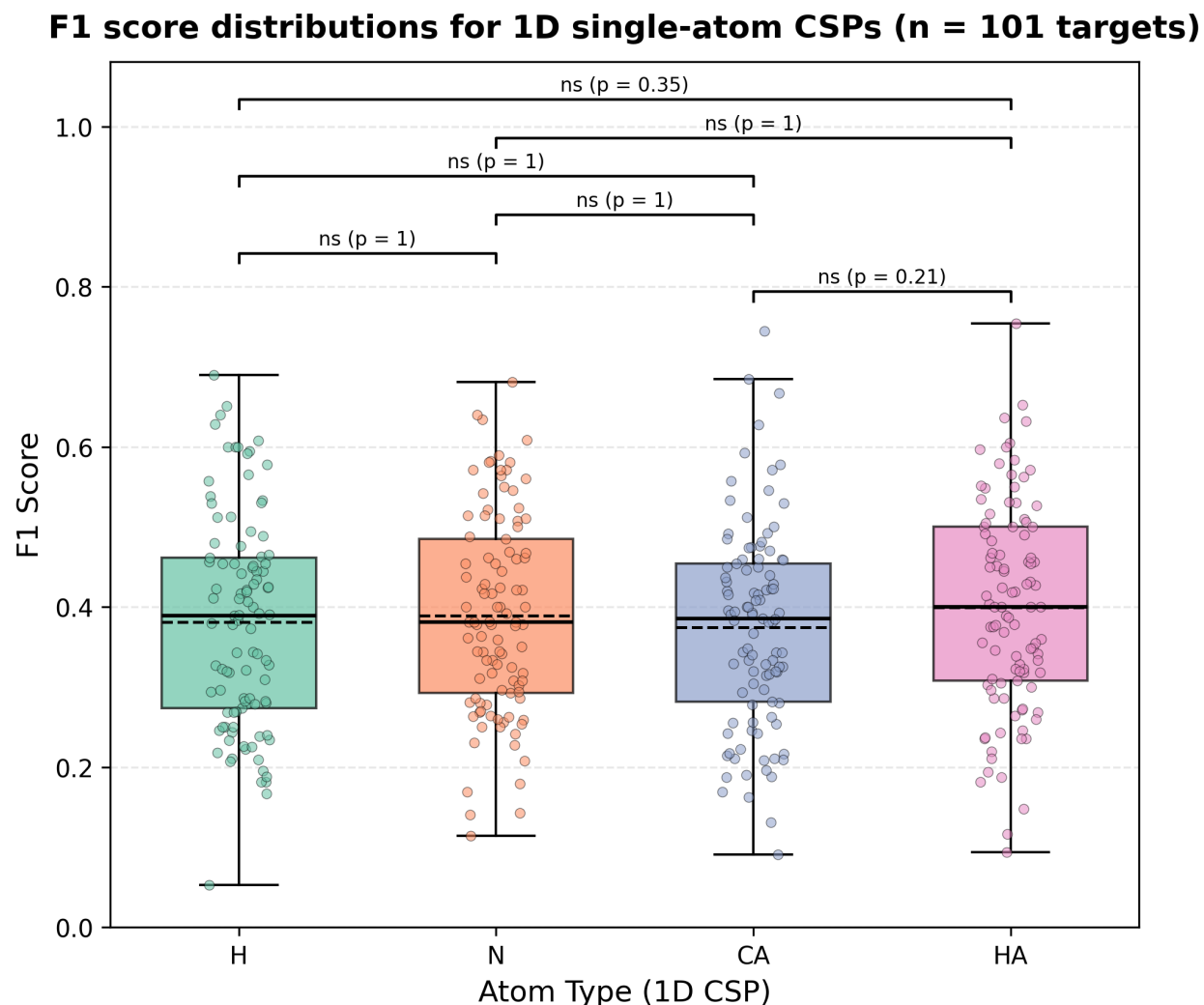
SI Fig. S15. Per-target F1 scores for 1D H/N/C \alpha /H \alpha CSPs ( n = 101 buffer-similar systems from CSP_UBQ_ph0.5_temp5C.csv with paired H/N/CA/HA F1 scores). Boxes show the per-target F1 distribution for 1D CSPs of each nucleus. Pairwise comparisons are two-sided Wilcoxon signed-rank tests for all unordered atom pairs, with Holm–Bonferroni adjustment of p -values. This figure shows there are no substantial differences in the distribution of F1 scores calculated based on 1D CSPs; distal CSPs occur for all types of atomic shifts at approximately the same frequency.
