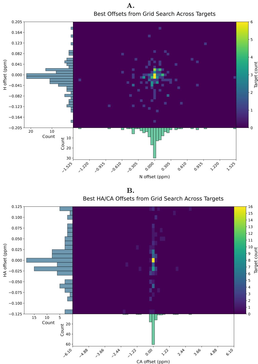
SI Fig. S21. Ideal chemical-shift offset grids for buffer-similar systems in CSP_UBQ_ph0.5_temp5C.csv with pipeline outputs. A. H/N referencing ( n = 135 ): a grid search selects the H/N offsets that maximize aligned HN peak counts under the pipeline CSP criterion; the heatmap aggregates those optimal ( \Delta\delta_N , \Delta\delta_H ) pairs (color = number of targets). Marginal histograms show the one-dimensional distributions of best H (left) and N (bottom) offsets. B. HA/CA referencing ( n = 101 systems with HA/CA grid-search CSVs): the same layout for offsets that maximize aligned HA/CA peak counts, with HA (left) and CA (bottom) marginals. Both nuclei pairs are peaked near zero, indicating that most apo/holo pairs require only small referencing corrections.
