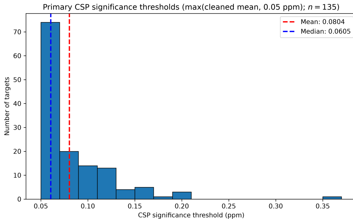
SI Fig. S23. Distribution of CSP significance thresholds (primary cutoff max(cleaned mean, 0.05 ppm); n = 135 buffer-similar systems from CSP_UBQ_ph0.5_temp5C.csv with pipeline outputs). Mean = 0.0804 ppm. This figure shows our mean CSP threshold is 0.08 ppm, corresponding to \sim 50 Hz at 600 MHz, which is 2–5 \times larger than the corresponding proton resonance linewidths.
