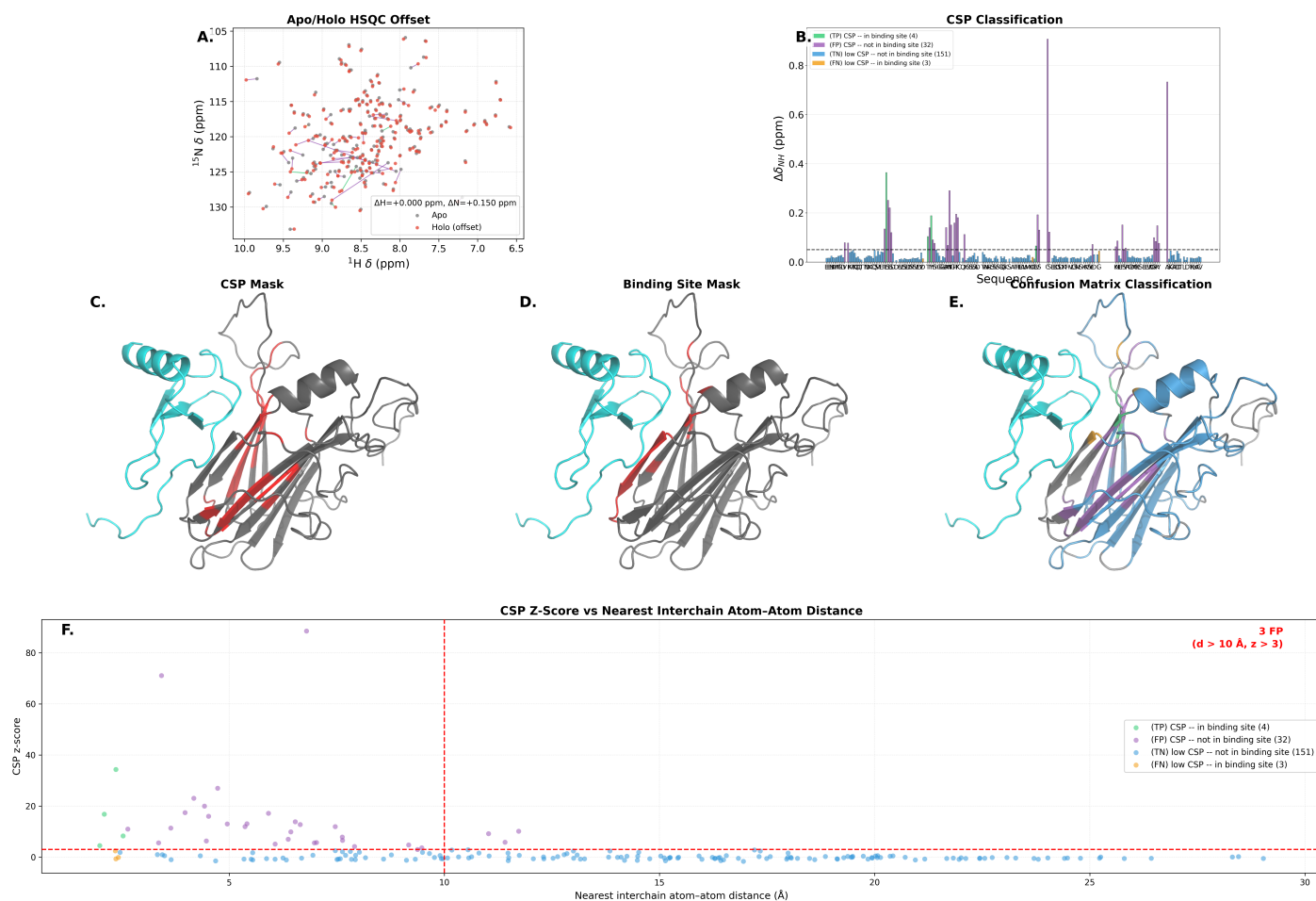
SI Fig. S18. Case study for holo 2FIN / apo BMRB 6809 (holo BMRB 7024). A. ^{15}\text{N}/^1\text{H} HSQC scatterplot overlaying the apo and holo assigned spectra with the optimal N/H offset applied. B. Calculated CSPs for receptor residues along the sequence, bars colored by confusion matrix classification. C. The mask of significant CSPs. D. The mask of binding-site residues. E. The confusion matrix classification projected onto the structure: distal CSPs are purple (FP), CSPs in the binding site are green (TP), non-CSPs in the binding site are orange (FN), and non-CSPs outside of the binding site are blue (TN). Residues without CSP measurements are shown in gray; ligands are colored cyan. F. CSP z versus nearest interchain atom-atom distance. Dashed lines mark z = 3 and d = 10 \text{ \AA} ; the annotation counts false positives with d > 10 \text{ \AA} and z > 3 . This plot shows monotonic decay of CSPs with increasing nearest interchain atom-atom distance. Residues in a set of \beta sheets further away from the ligand with significant shifts have lower CSPs than those closer to the binding site.
