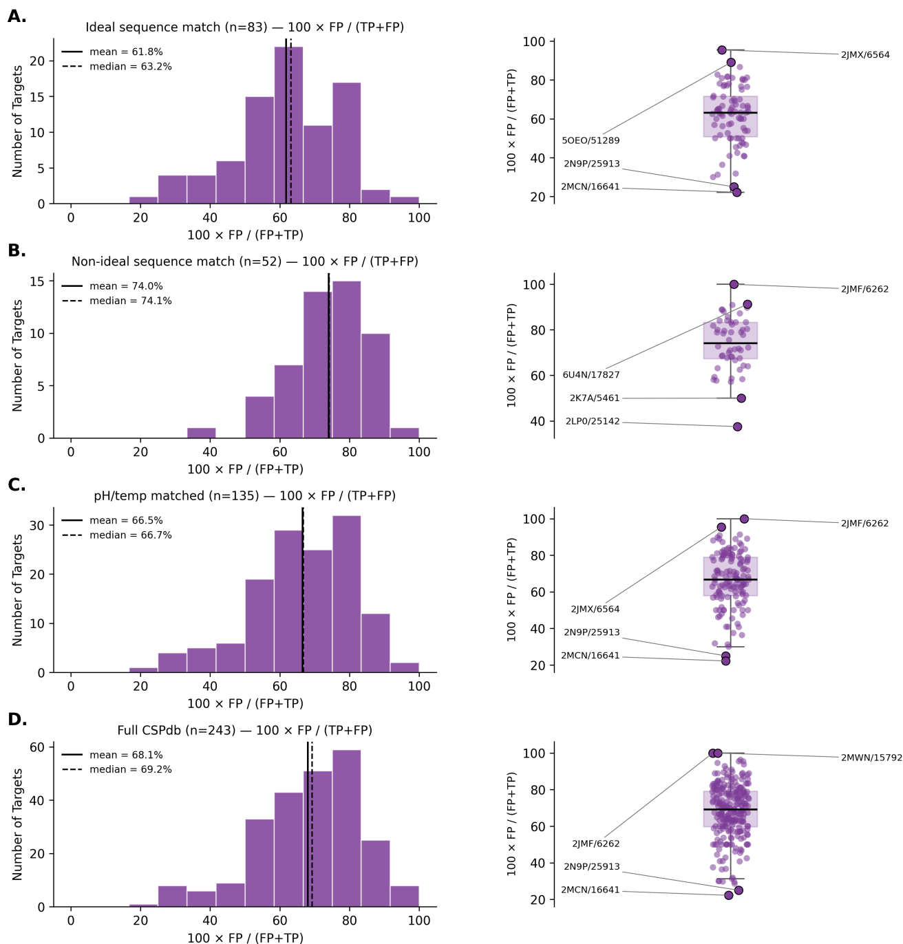
SI Fig. S16. Per-target false-positive rates under the primary CSP cutoff max(cleaned mean, 0.05 ppm). A. ideal sequence match ( n = 83 ); B. non-ideal sequence match ( n = 52 ); C. pH/temp matched ( n = 135 ); D. full CSPdb ( n = 243 ). For each cohort, panels report 100 \times \text{FP} / (\text{TP} + \text{FP}) among significant CSPs. This figure shows per-target false positive rates across four subsets, and reveals there are minimal differences between these four subsets.
