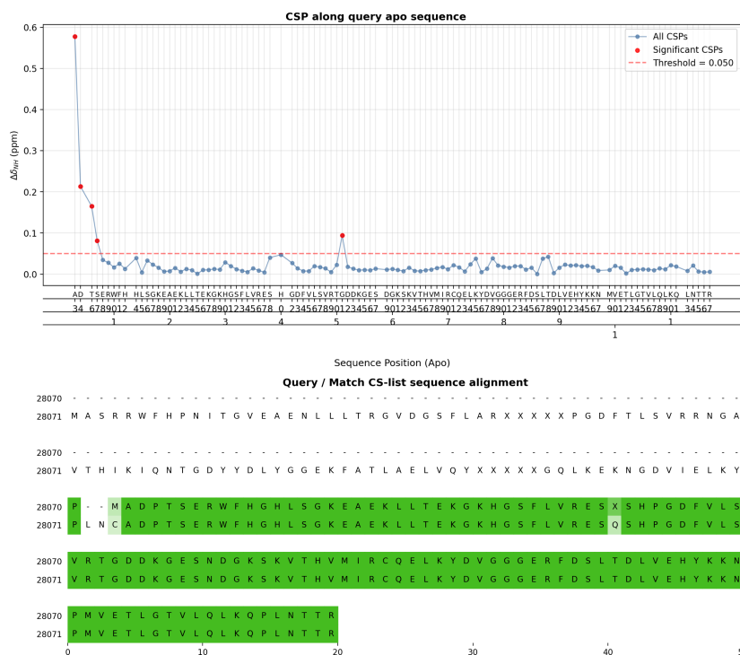
SI Fig. S25B. Apo vs apo control study for BMRB 28070 and 28071. This case involves the SH2 domains of SHP2. BMRB 28071 is the tandem nSH2–cSH2 construct and includes a large N-terminal region (the nSH2 domain and inter-SH2 linker, ~100 residues) that is absent from the isolated cSH2 entry (BMRB 28070). 95.4% of the CSPs for this control are below 0.05 ppm.
