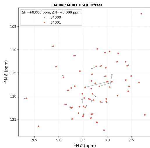
SI Fig. S25C. Apo vs apo control study for BMRB 34000 and 34001. This case involves insulin-like growth factor II (IGF-II). BMRB 34001 is the [S39_PQ]-IGF-II variant and contains a two-residue Pro-Gln insertion after Ser39 relative to wild-type IGF-II (BMRB 34000). 90.6% of the CSPs for this control are below 0.05 ppm.
