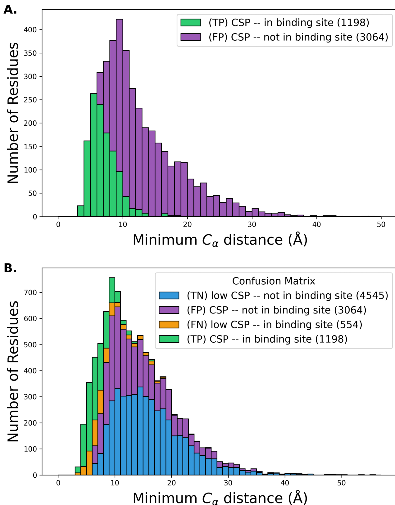
SI Fig. S10. HA/CA CSP confusion histograms for the buffer-similar systems from CSP_UBQ_ph0.5_temp5C.csv that also have H\alpha and C\alpha shifts in both apo and holo experiments ( n = 101 ). These results are very similar to CSPs calculated using SI Equation S1. 71.9% of CSPs using SI Equation S3 are distant from the binding site compared to 69.4% using SI Equation S1.
