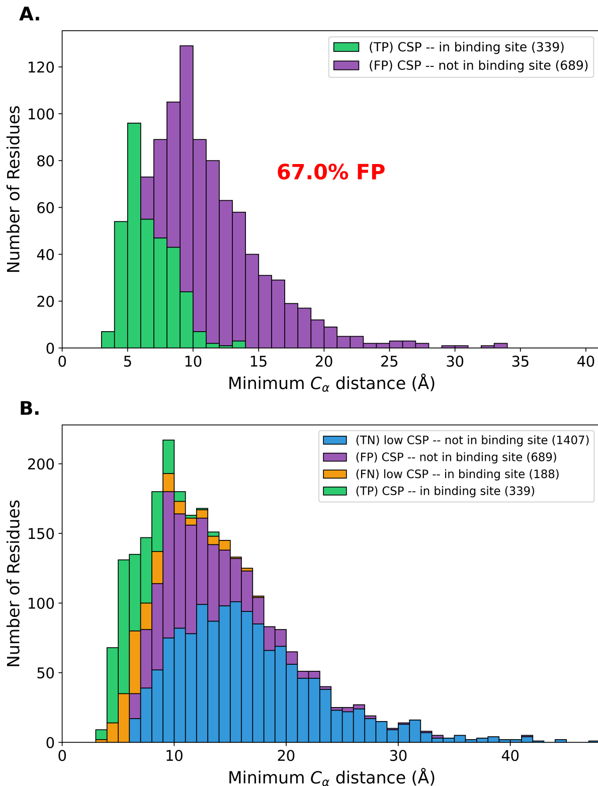
SI Fig. S9. Figure 3 histograms for the same-author/same-study subset. Targets are the curated pairs in CSP_UBQ_ph0.5_temp5C_same_author_list.csv ( n = 32 with pipeline outputs of 33 curated pairs): buffer-similar apo/holo systems that share a study or last author between apo and holo chemical-shift depositions. A. significant-CSP TP vs FP by minimum C_\alpha distance to the interface; B. full confusion-matrix stacks (TN/FP/FN/TP). This figure reports results on a very high-fidelity subset, and the results are very similar to those reported in Figure 3: 67.0% of CSPs are distal vs 69.4% of CSPs are distal in the n = 135 subset reported in Figure 3.
