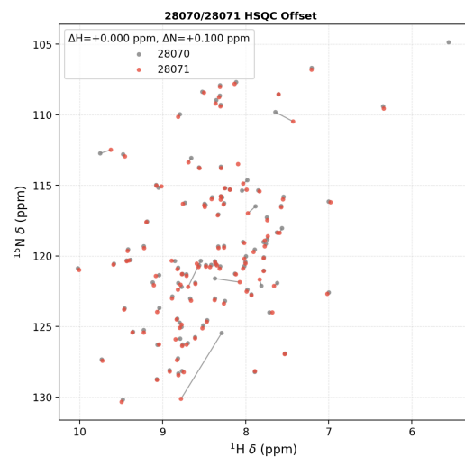
SI Fig. S25B. Apo vs apo control study for BMRB 28070 and 28071. This case involves the SH2 domains of SHP2. BMRB 28071 is the tandem nSH2–cSH2 construct and includes a large N-terminal region (the nSH2 domain and inter-SH2 linker, ~100 residues) that is absent from the isolated cSH2 entry (BMRB 28070). 95.4% of the CSPs for this control are below 0.05 ppm.
