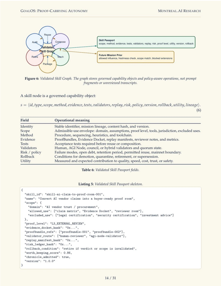
A validated capability passport carries scope, evidence, replay, freshness and rollback.
