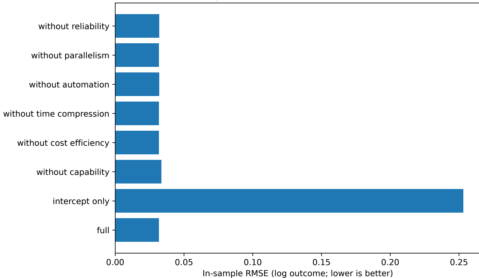
Synthetic canonical-model ablations
