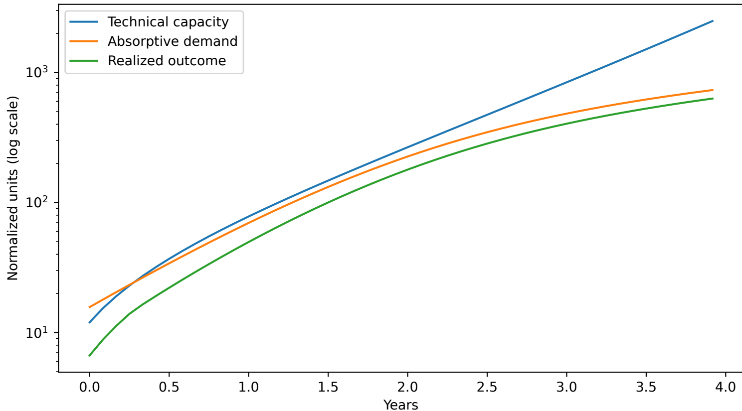
The canonical model separates capacity, absorption, and realization
