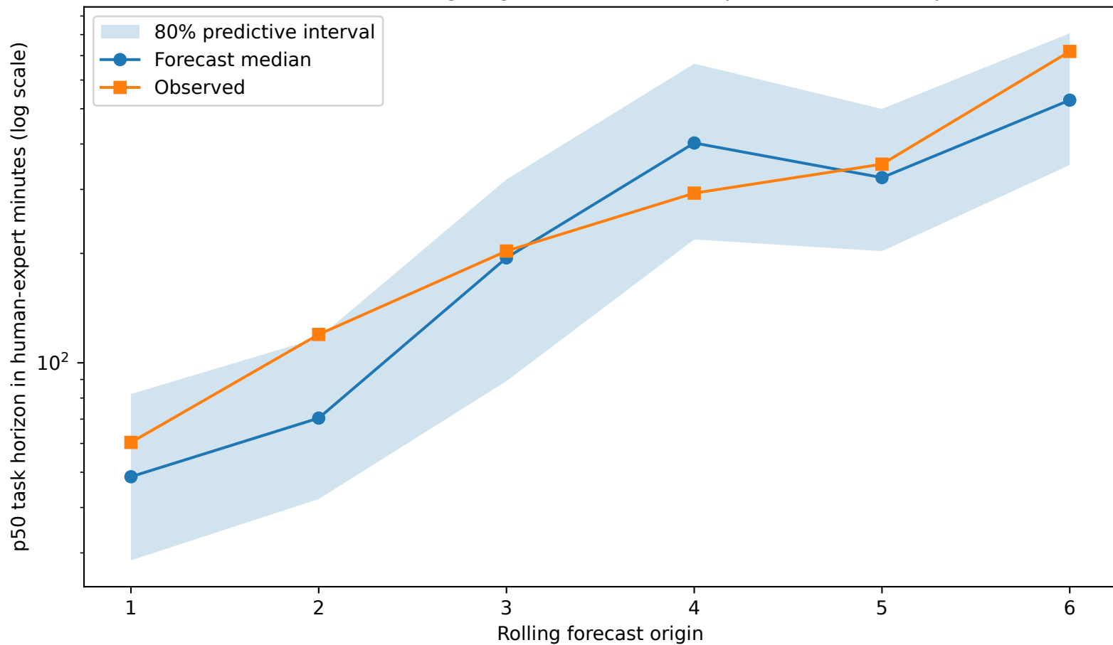
Probabilistic rolling-origin hindcast on the public METR excerpt
