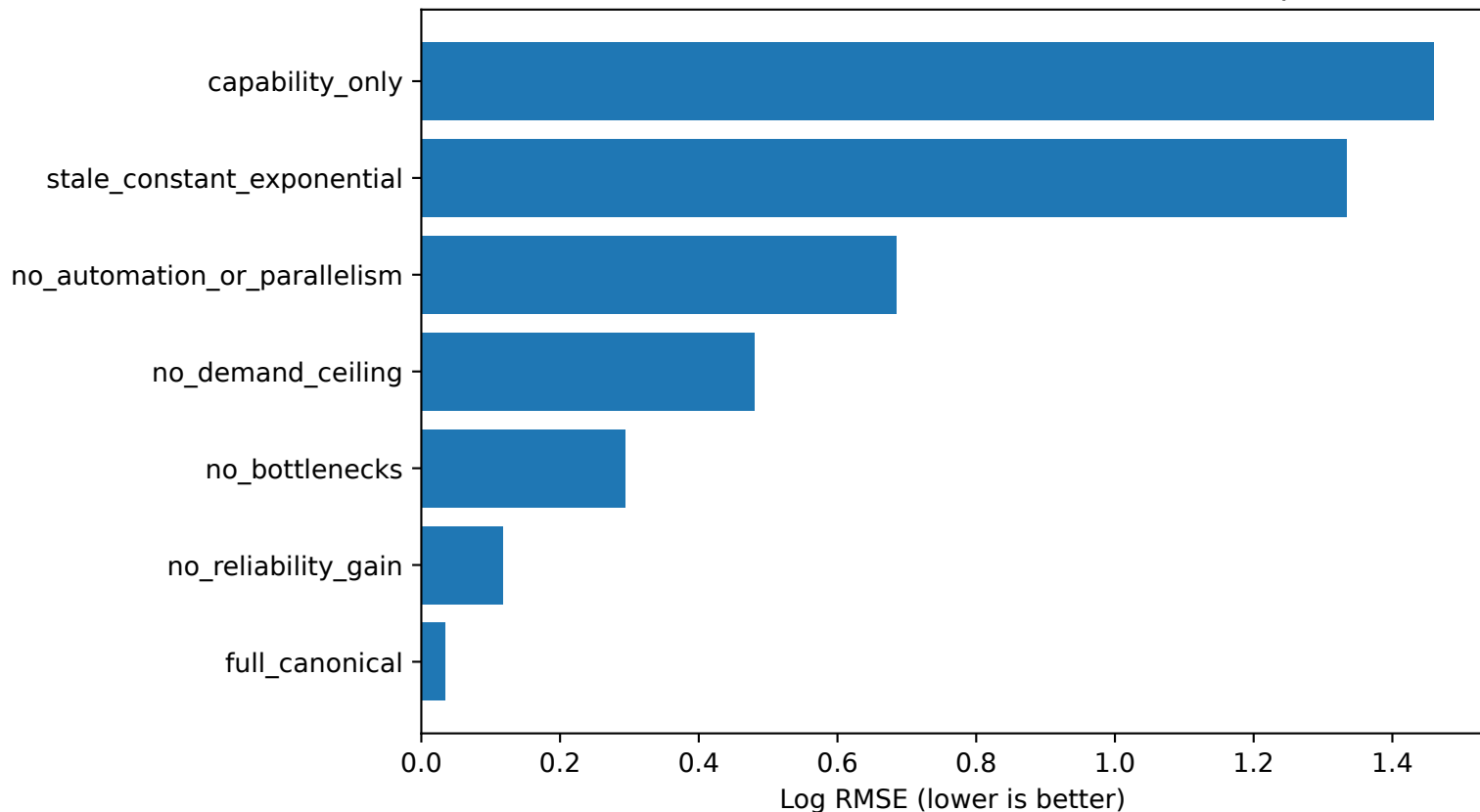
Ablation error in the controlled canonical-model experiment
