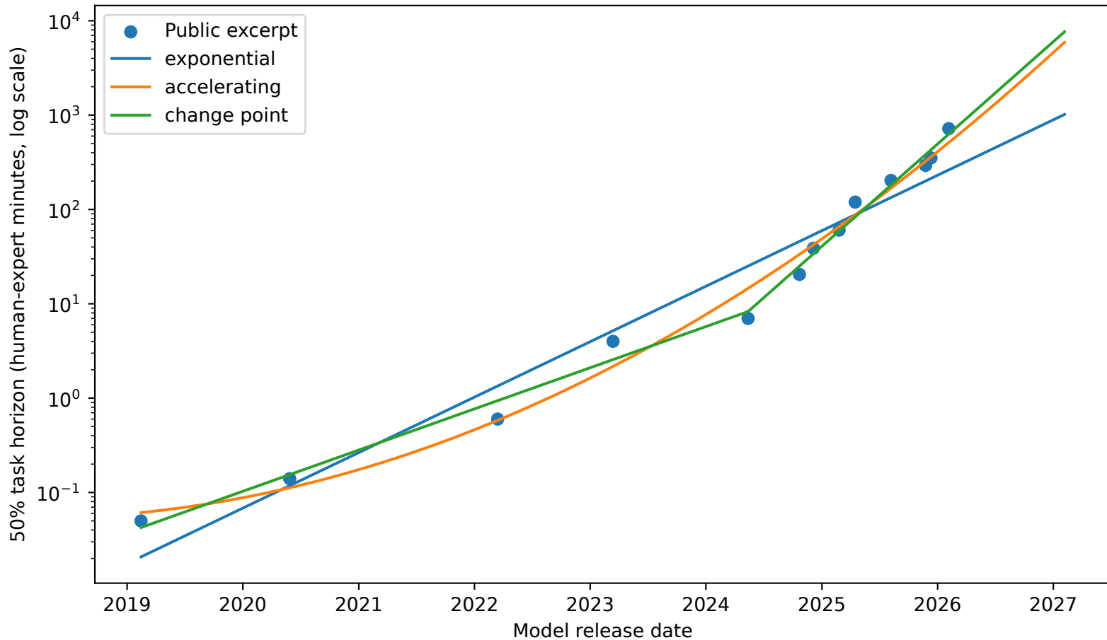
Illustrative model fits to a public METR excerpt
