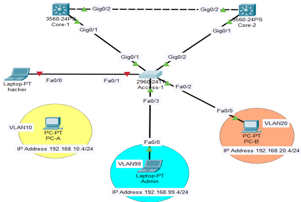
Figure 4.8: Port Security Violation Triggered by Rogue Device
