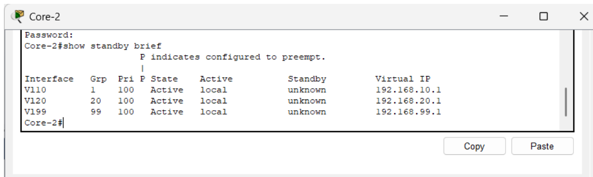
Figure 4.6: Core-2 Transition to Active State Post-Failure
