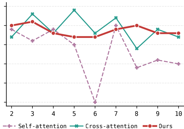
(b) Attention-based fusion
