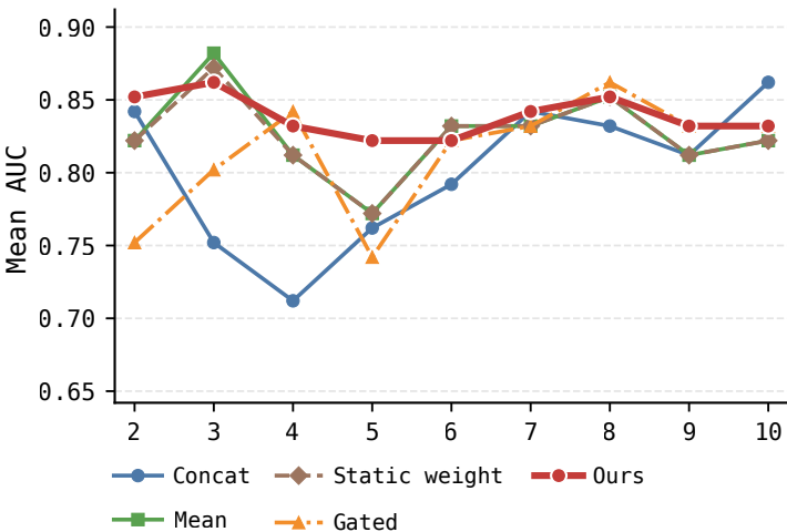
(a) Aggregation and weighting
