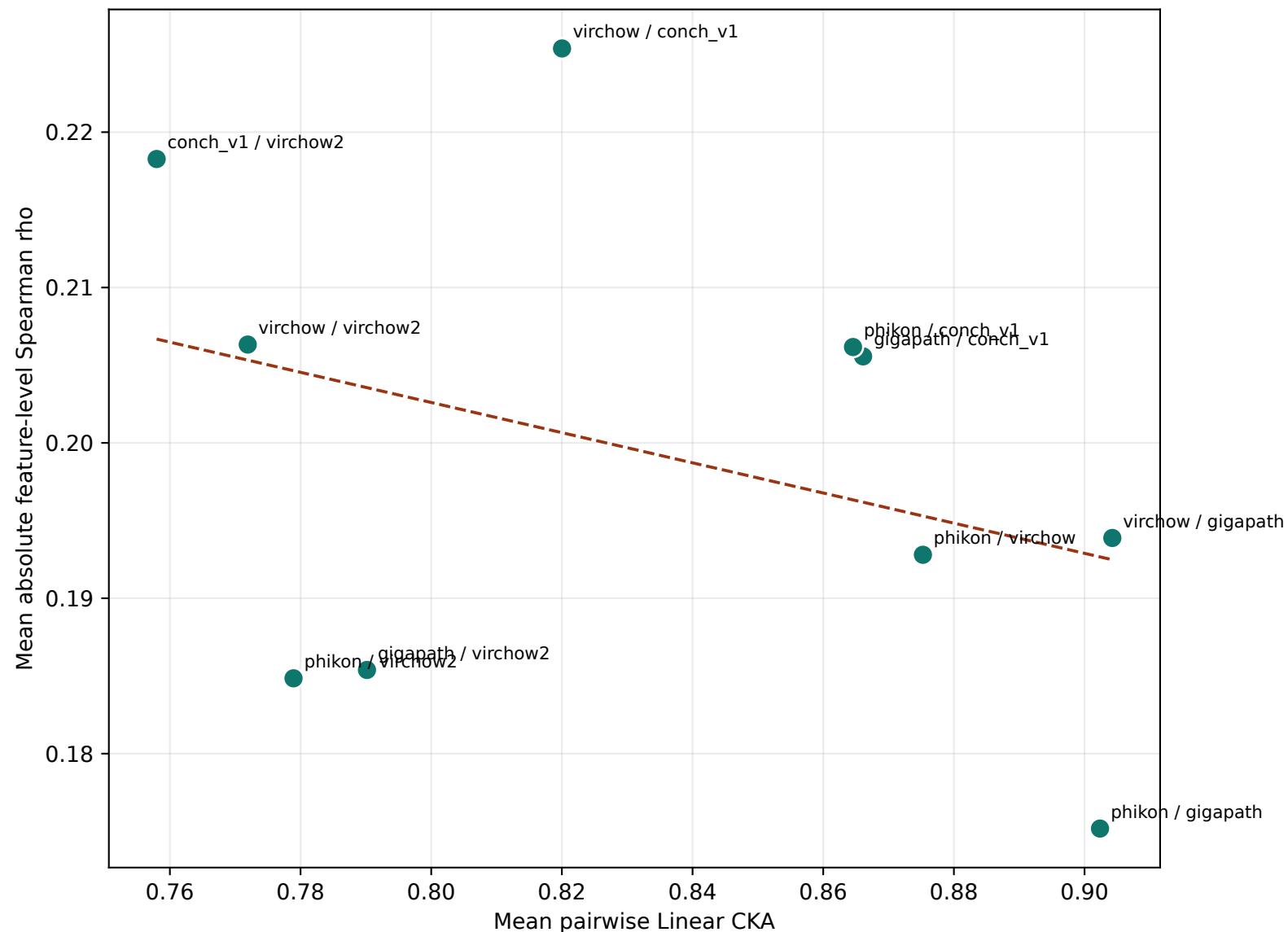
CKA and feature-level Spearman correspondence Pairs=10 | Pearson r=-0.344 | Spearman \rho=-0.418 , p=0.229
