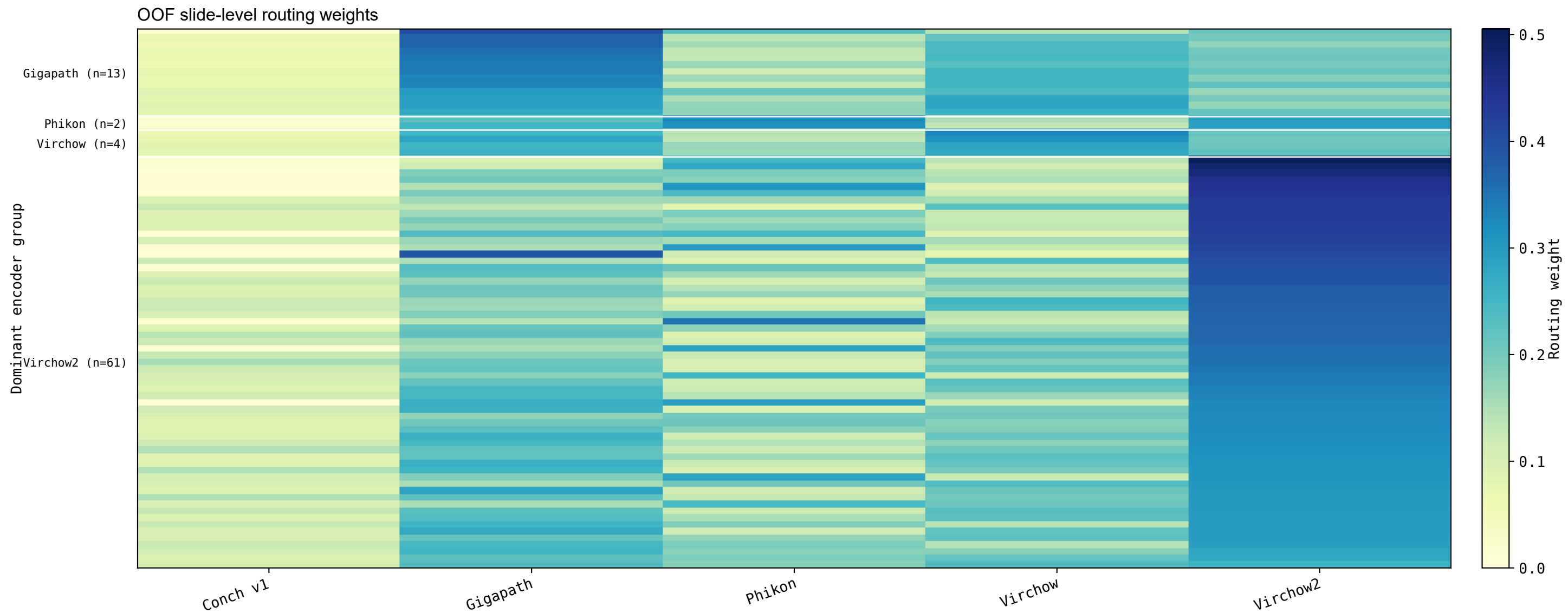
GME Out-of-Fold Routing-Weight Distribution
