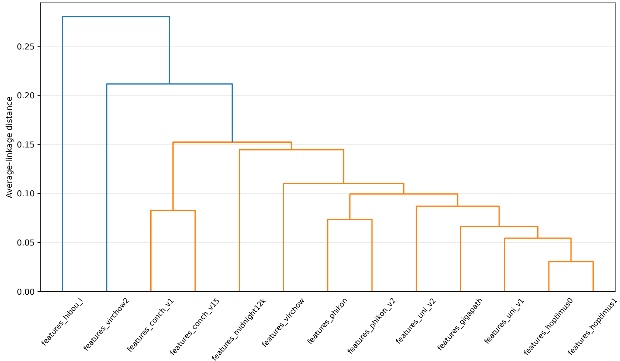
Foundation Model Clustering from 1 - Linear CKA
