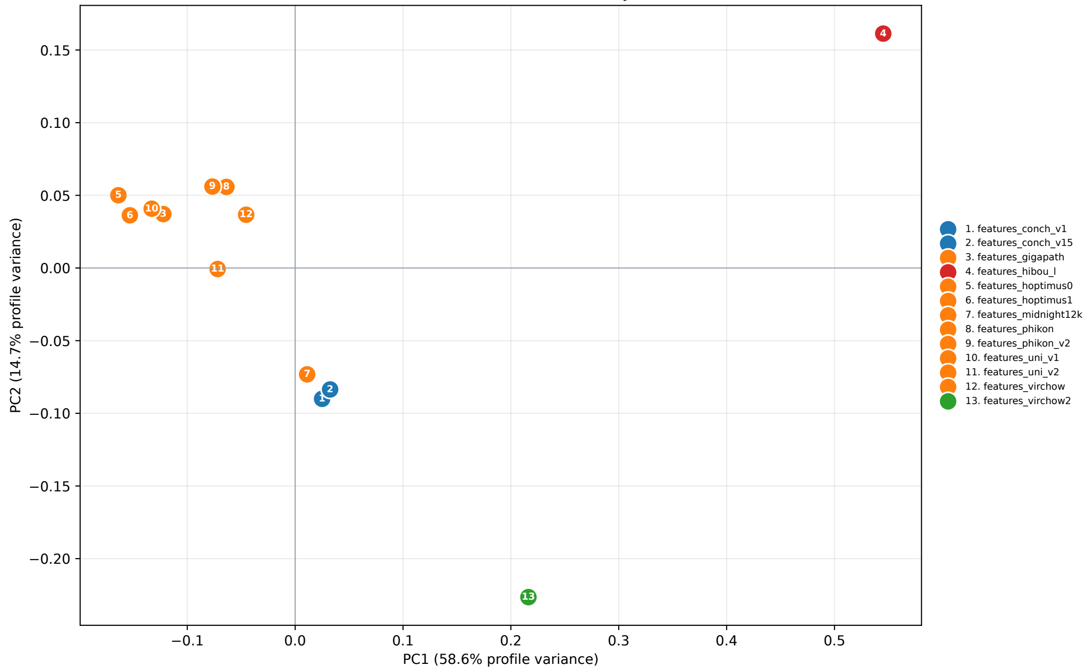
PCA of Foundation-Model CKA Similarity Profiles
