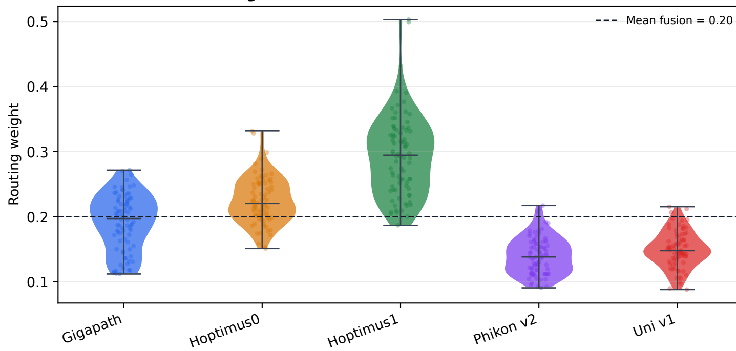
Encoder-wise OOF weight distributions
