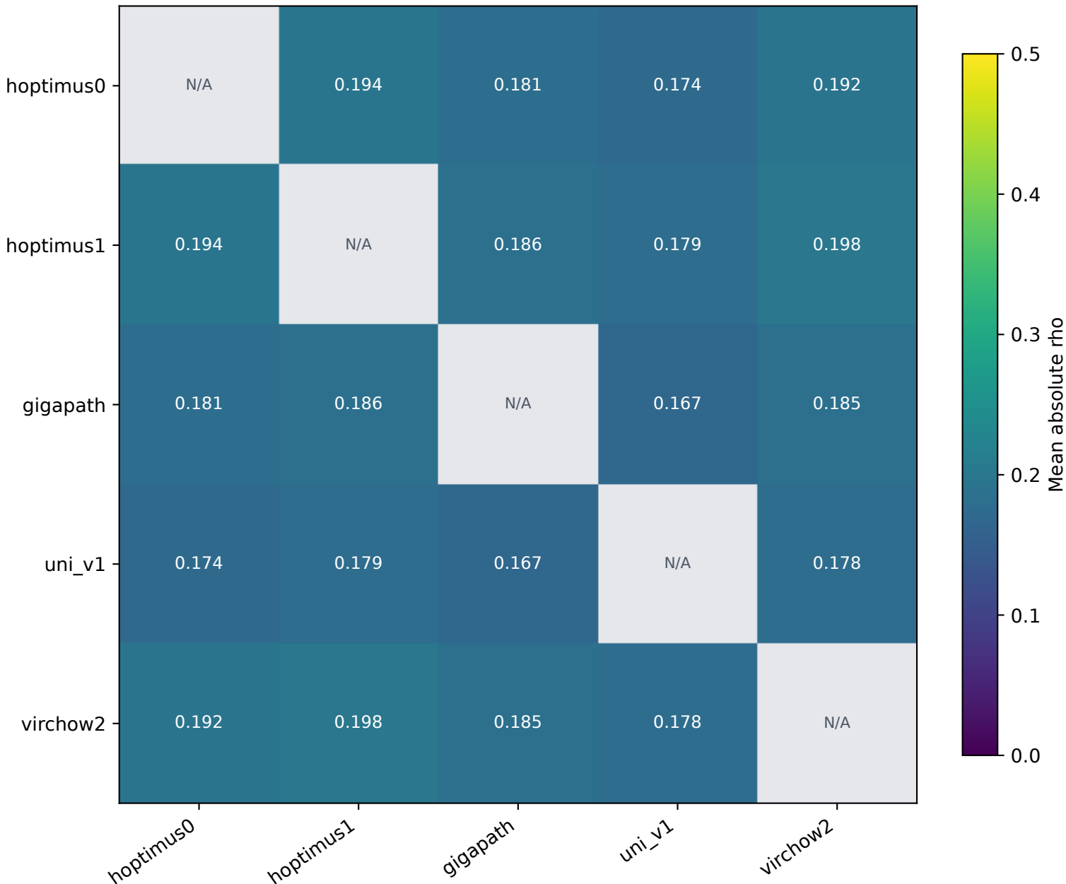
Mean absolute feature-level Spearman correlation
