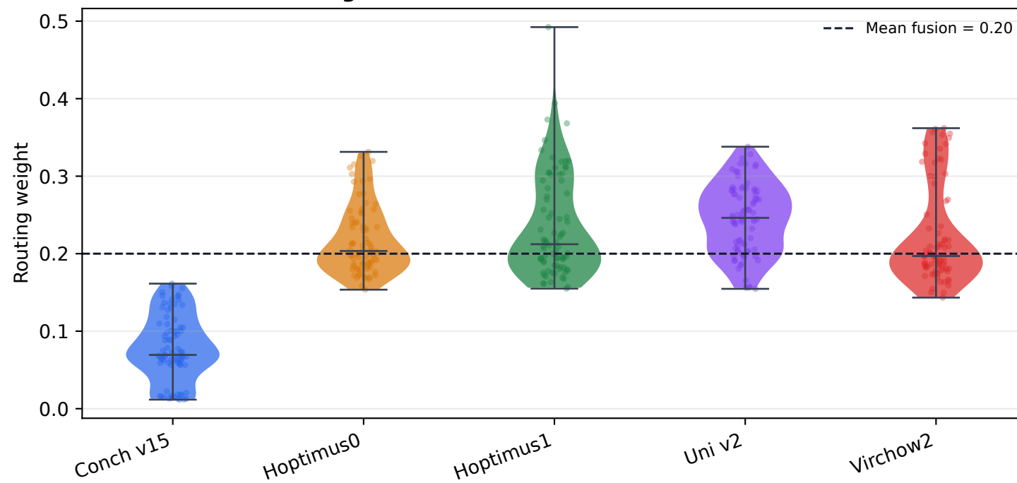
Encoder-wise OOF weight distributions
