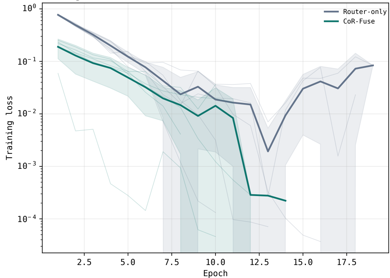
Training loss
