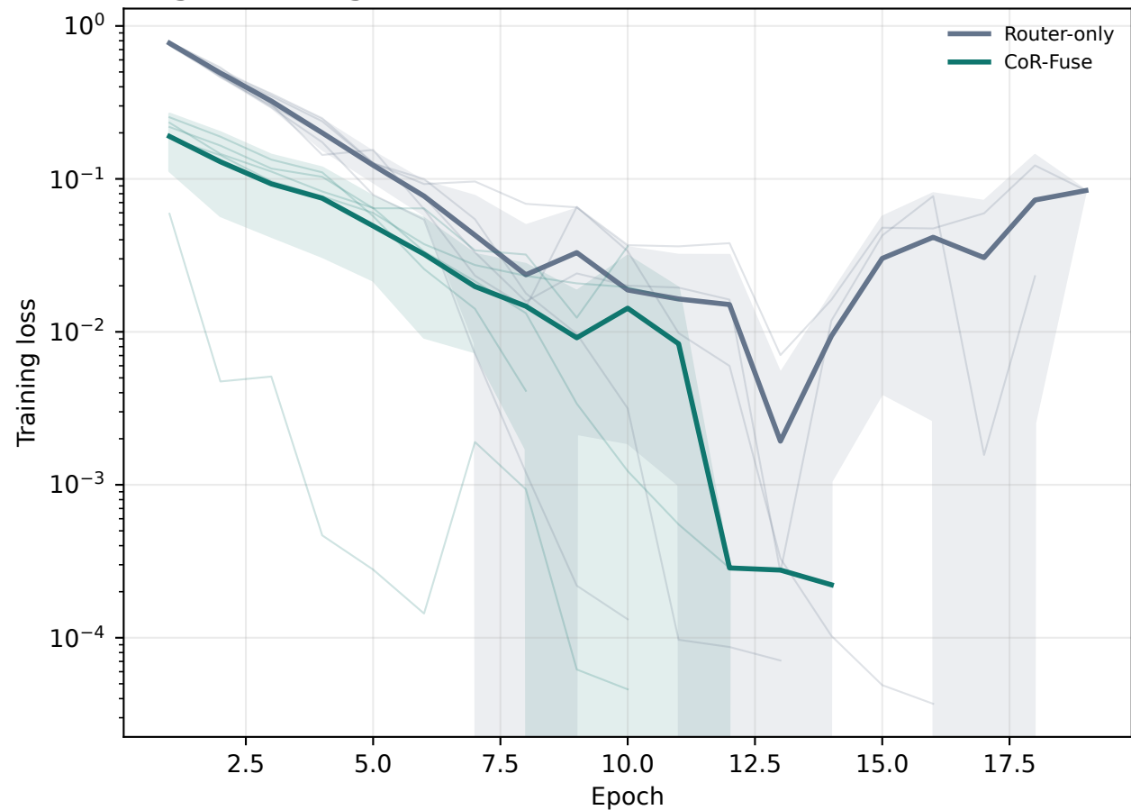
Stage-2 training loss
