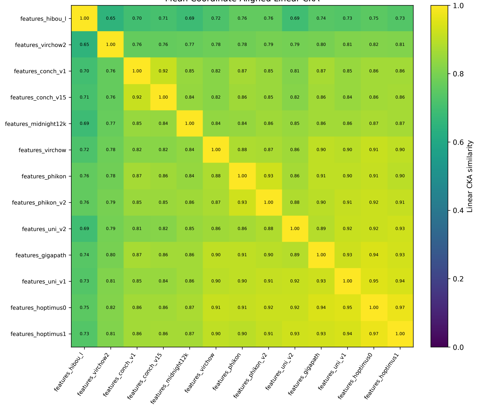
Mean Coordinate-Aligned Linear CKA
