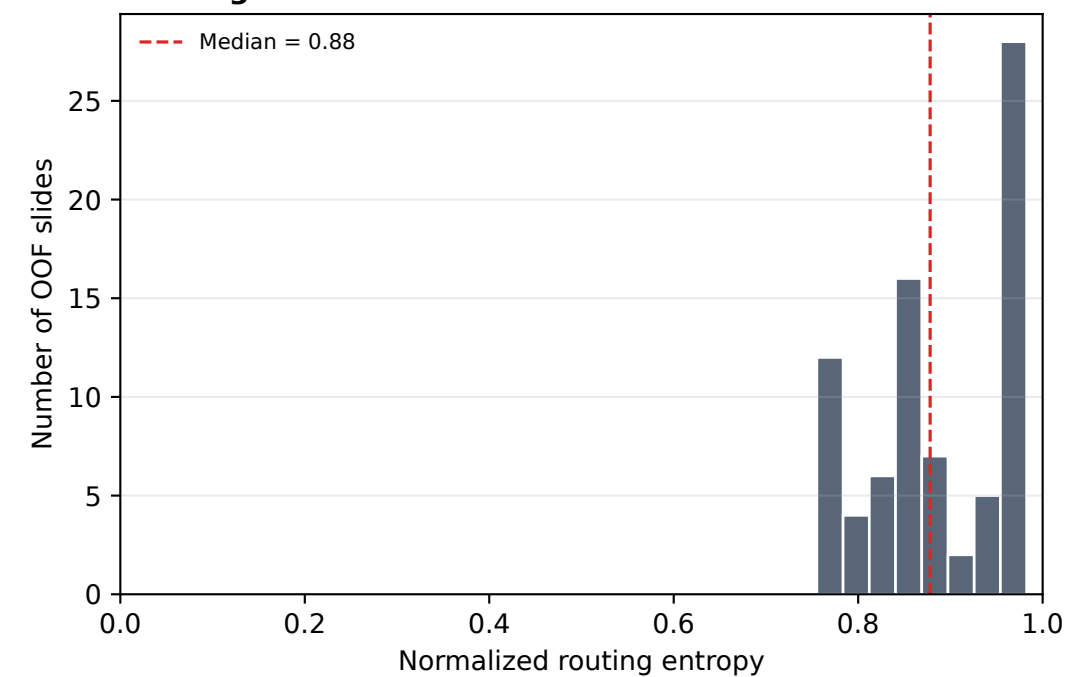
Routing concentration across slides
