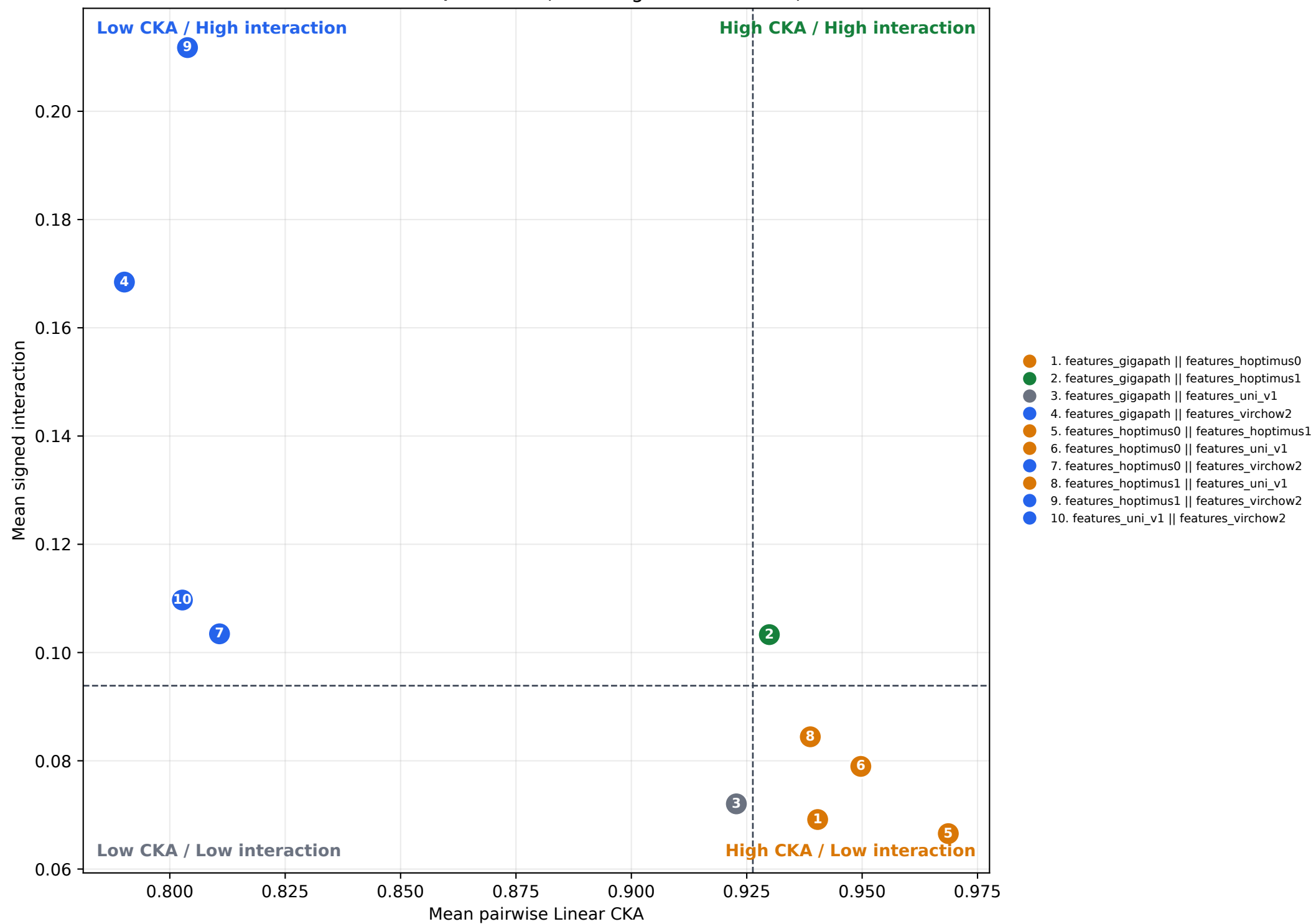
CKA-Interaction Quadrants (mean signed interaction)
