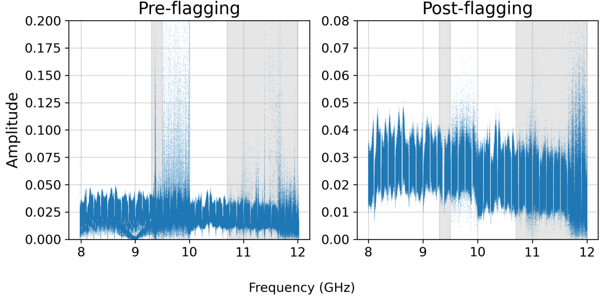
Figure 3.2: Frequency versus amplitude of the raw primary calibrator visibilities before (left) and after (right) a priori and AOFLAGGER flagging. Note the different y-axis scales between panels. Known high-RFI regions are shaded in grey. Data is shown for all baselines. Residual shape in the post-flagging data is primarily due to the absence of the bandpass correction (e.g. Figure 3.3).
