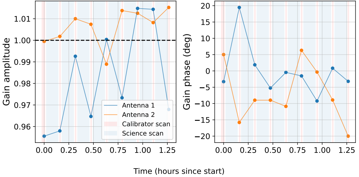
Figure 3.4: Example complex gain calibration. Amplitude (left) and phase (right) solutions for a single polarisation and spectral window are shown for two representative antennas over the course of an observation. Red shaded regions mark secondary calibrator scans, interleaved between blue shaded science target scans.
