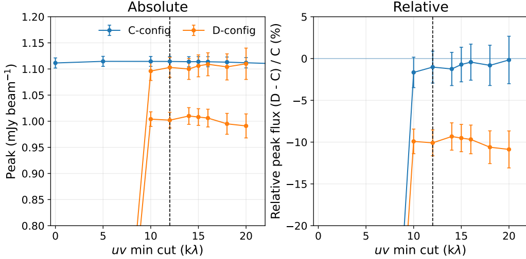
Figure 4.2: Flux density fit for RXJ1720+2638 BCG as a function of minimum uv -range used during imaging. The black vertical line indicates the adopted minimum uv -cut. Left Panel: Absolute peak flux with 1\sigma error for each dataset. Right Panel: Relative peak flux density of D-configuration to C-configuration.
