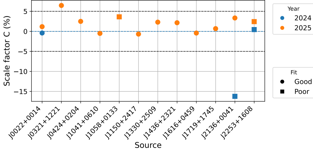
Figure 4.4: Month-to-month broadband variation for all secondary calibrators. The year of measured variation is denoted by colour. A good fit (circles) corresponds to highly linear broadband scaling, while a poor fit (squares) indicates changes in spectral shape. The adopted calibration uncertainty (5%) is marked for comparison.
