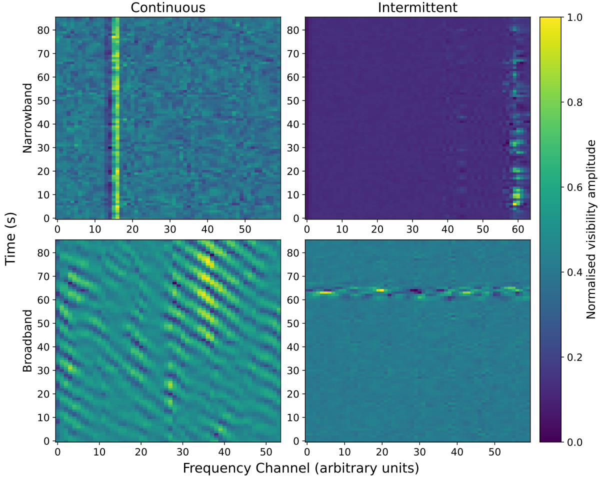
Figure 3.1: Examples of RFI in time–frequency space for a representative baseline. Columns show continuous and intermittent behaviour, while rows show narrowband (top: representative \sim 128 MHz sub-bands within 9.3–9.9 GHz, likely associated with satellite and weather radar emissions) and broadband RFI (bottom: representative \sim 128 MHz sub-bands within 10.7–12 GHz, likely associated with ground-based links and geostationary satellites).
