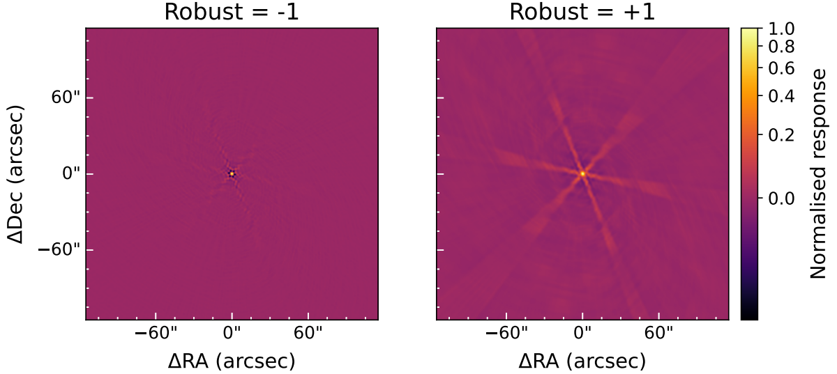
Figure 3.6: Example point spread functions for imaging with Briggs weighting robust = -1 (more uniformly weighted; left) and robust = 1 (more naturally weighted; right). Both images are normalised to a peak value of 1 and shown on a common colour scale to illustrate the difference in sidelobe prominence.
