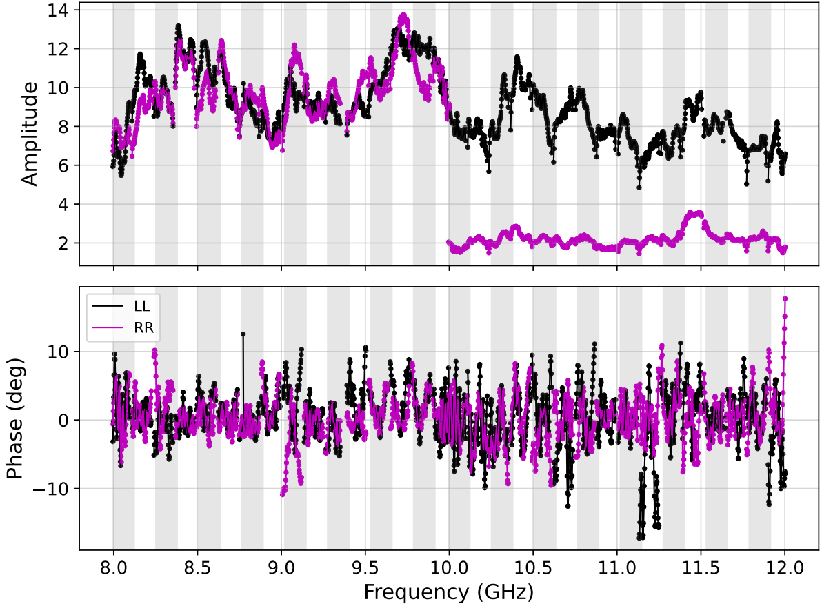
Figure 3.3: Example bandpass calibration. Amplitude (top) and phase (bottom) time-independent solutions are shown for the parallel-hand (LL, RR) correlations of a single antenna. Spectral windows are indicated by alternating grey shaded regions to highlight discontinuities at their boundaries. The pronounced discontinuity in the RR correlation at 10 GHz marks the baseband transition between 8–10 and 10–12 GHz.
