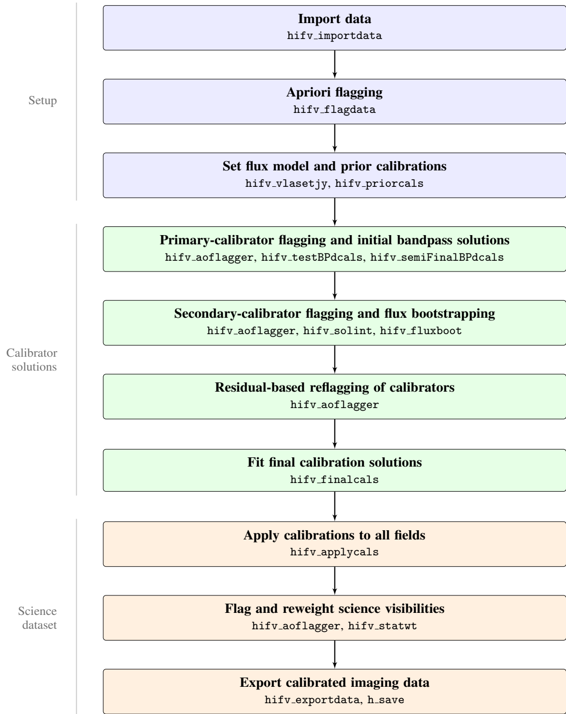
Figure 3.2: Overview of the modified CASA calibration pipeline. Each step includes the related CASA functions.
