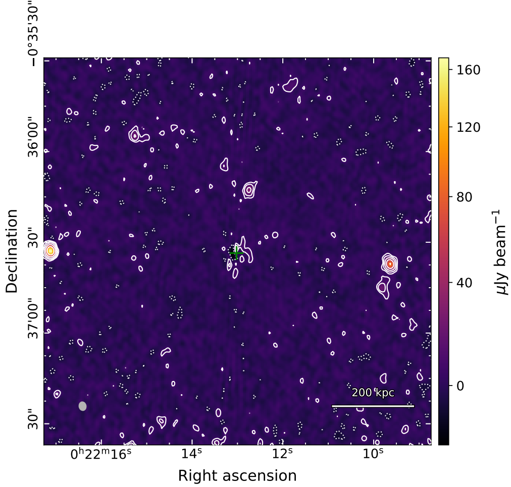
Figure 5.22: ACTJ0022-0036. Point source subtracted and primary beam corrected ( \text{robust} = 1 ) 10 GHz image with a restoring beam 2.90'' \times 2.36'' at a position angle of -10.7^\circ (shown in grey, bottom left) and an rms noise of 1.94 \mu\text{Jy beam}^{-1} . White contours are spaced by factors of two, starting from 3\sigma , with negative contours at -3\sigma shown as white dotted lines. The green cross marks the location of the subtracted source.
