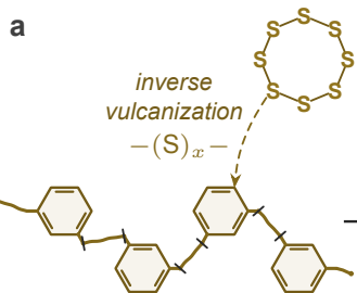
Sulfur-rich polymer poly(S-r-DIB) linear copolymer
