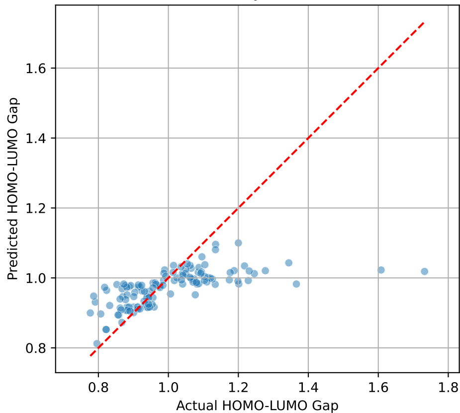
Parity Plot
