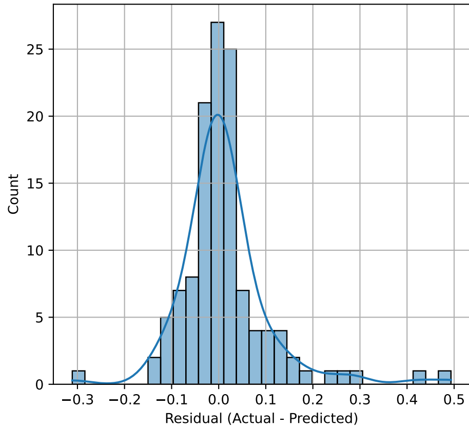
Residuals Histogram
