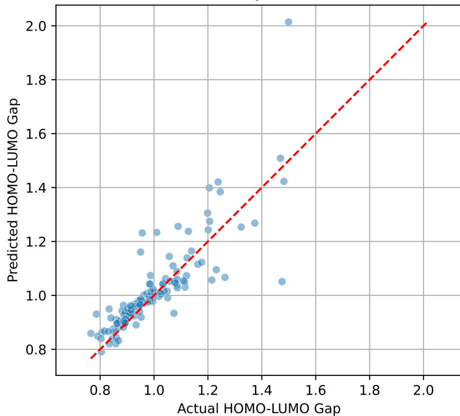
Parity Plot
