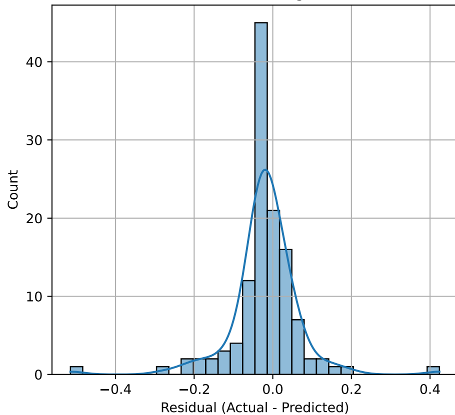
Residuals Histogram
