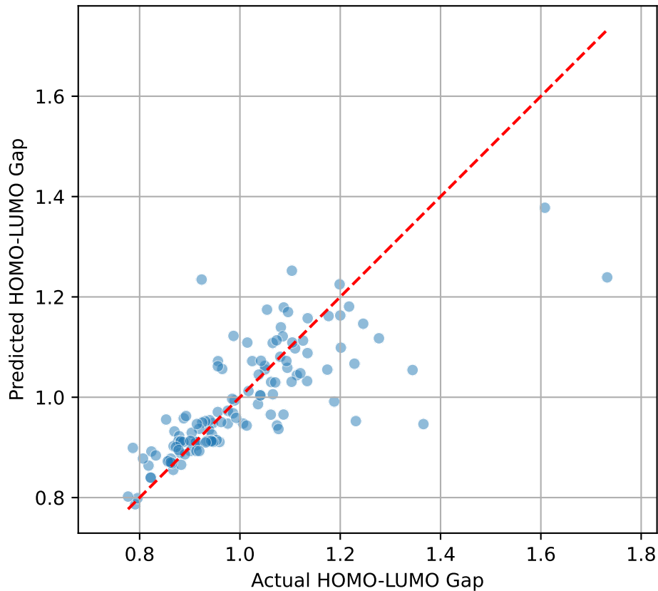
Parity Plot
