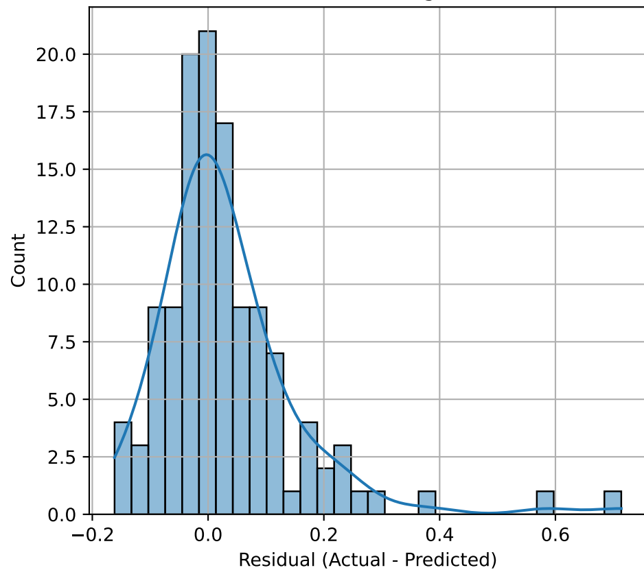
Residuals Histogram
