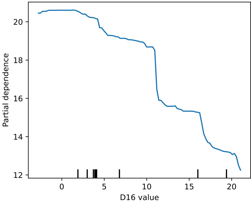
G Gradient Boosting — \Theta (dihedral angle)
