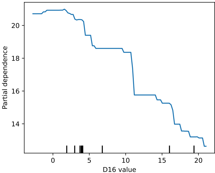
J Support Vector Regression — \Theta (dihedral angle)
