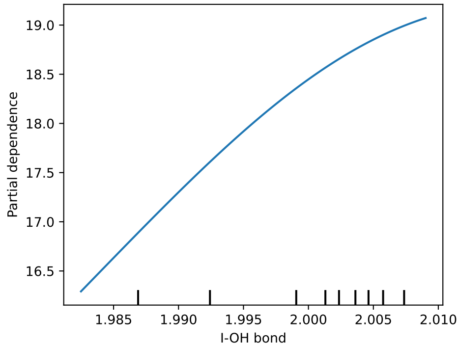
N Neural Network — I-OH bond length
