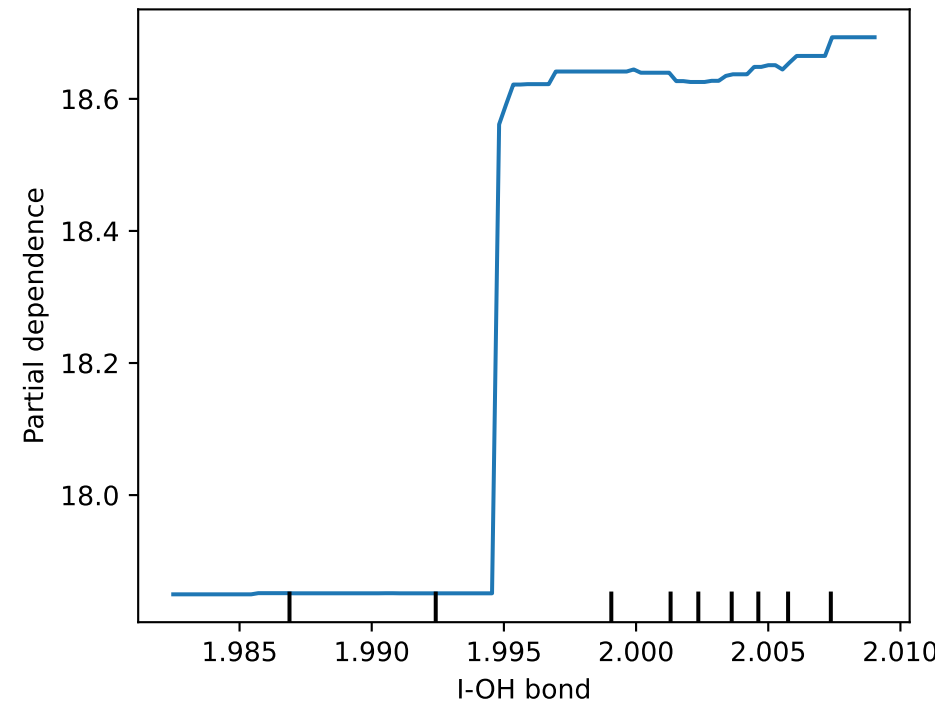
L Support Vector Regression — I-OH bond length
