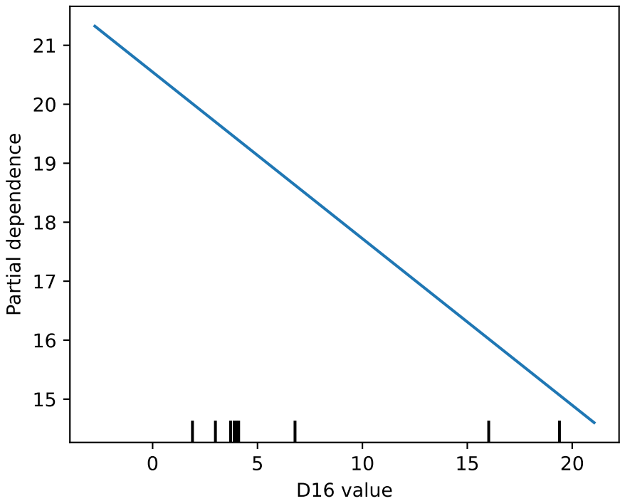
D Random Forest — \Theta (dihedral angle)
