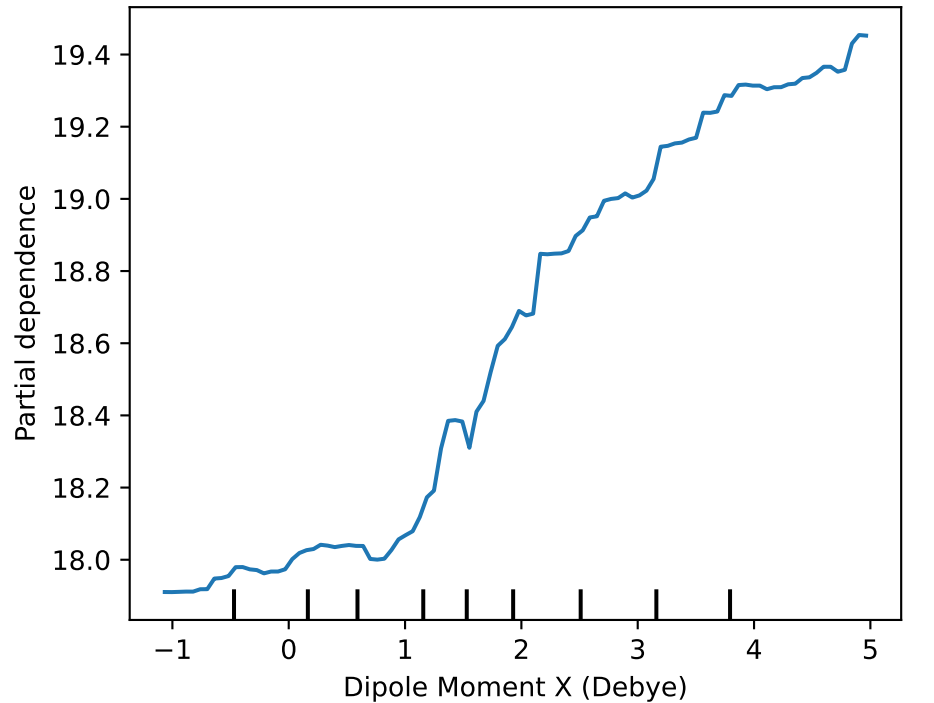
H Gradient Boosting — \mu_X (dipole moment, X)
