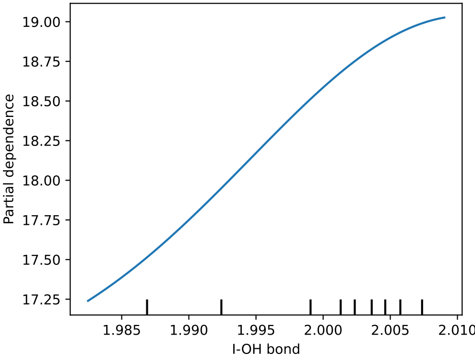
O Neural Network — \mu_X (dipole moment, X)
