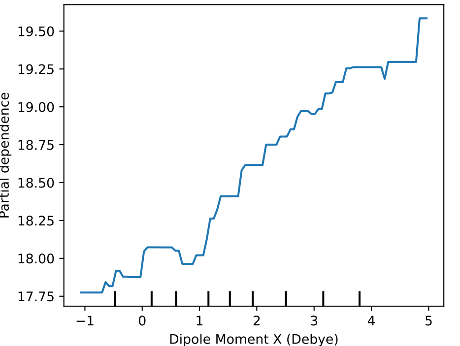
K Support Vector Regression — \mu_X (dipole moment, X)
