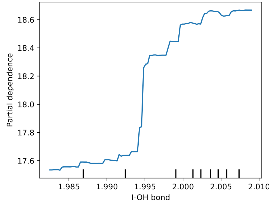
I Gradient Boosting — I-OH bond length
