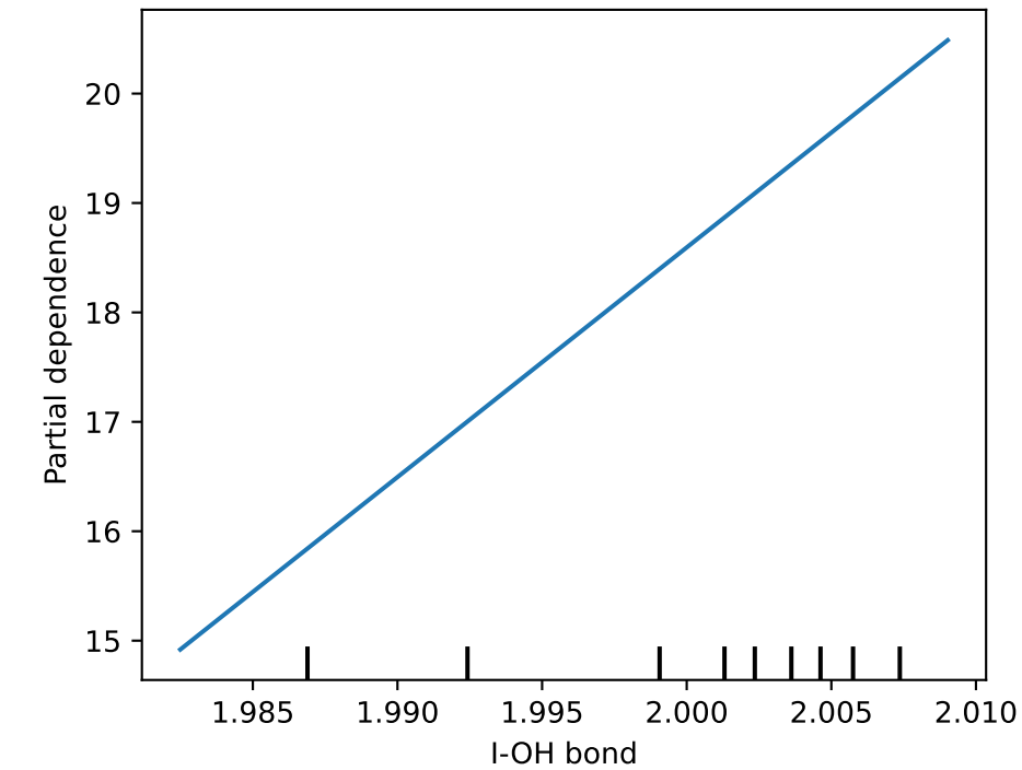
E Random Forest — \mu_X (dipole moment, X)
