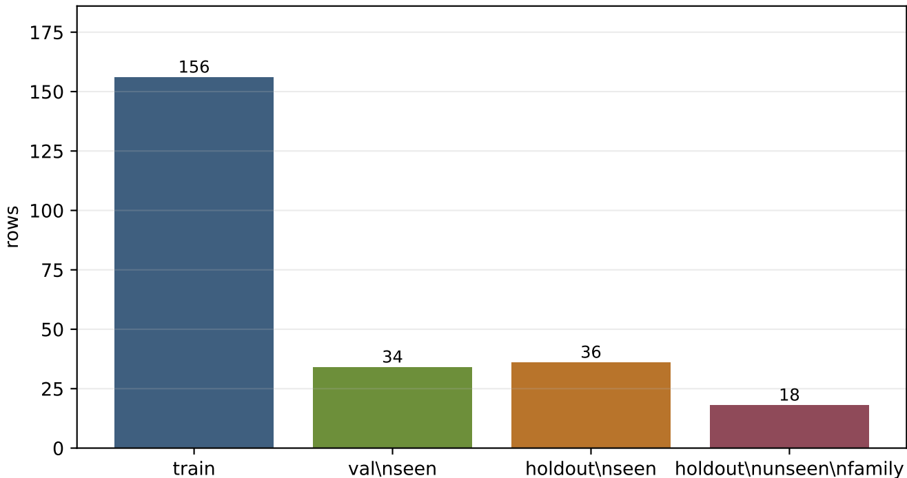
Leakage-aware near-miss repair split
