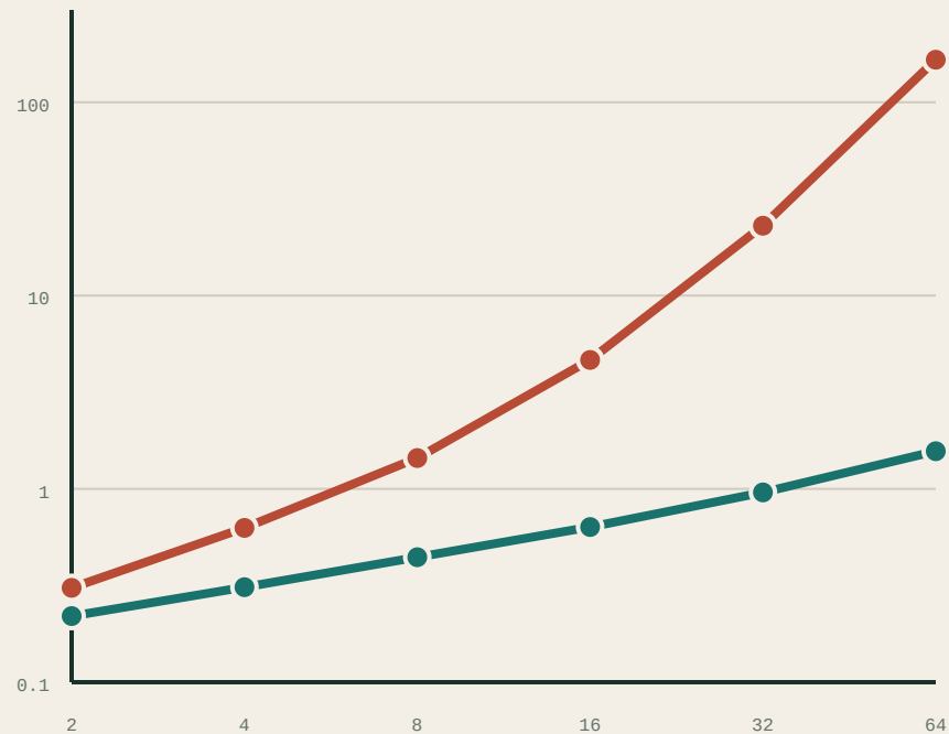
maximum gradient norm (log scale)
