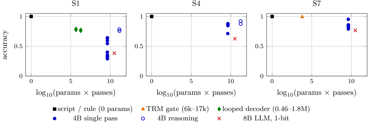
Figure 2: Accuracy against \log_{10}(\text{resident parameters} \times \text{sequential passes}) , one mark per arm family; parameter-free gates are plotted at 0. Registered arms only; seed replicates and the learning-rate control are in the repository’s addenda table.
