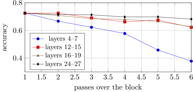
Figure 1: Zero-shot recurrence, choice readout, 400 dev items. One pass is the unmodified model. Each point is read from a single six-pass run through the tail lens.
