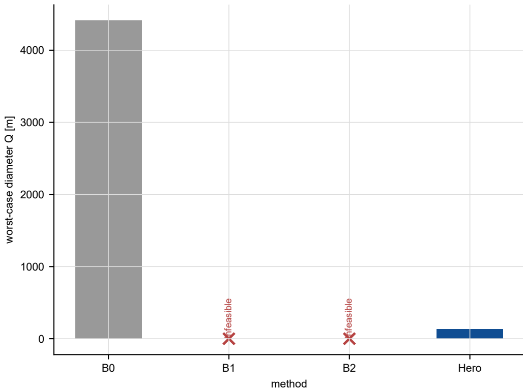
baseline comparison
