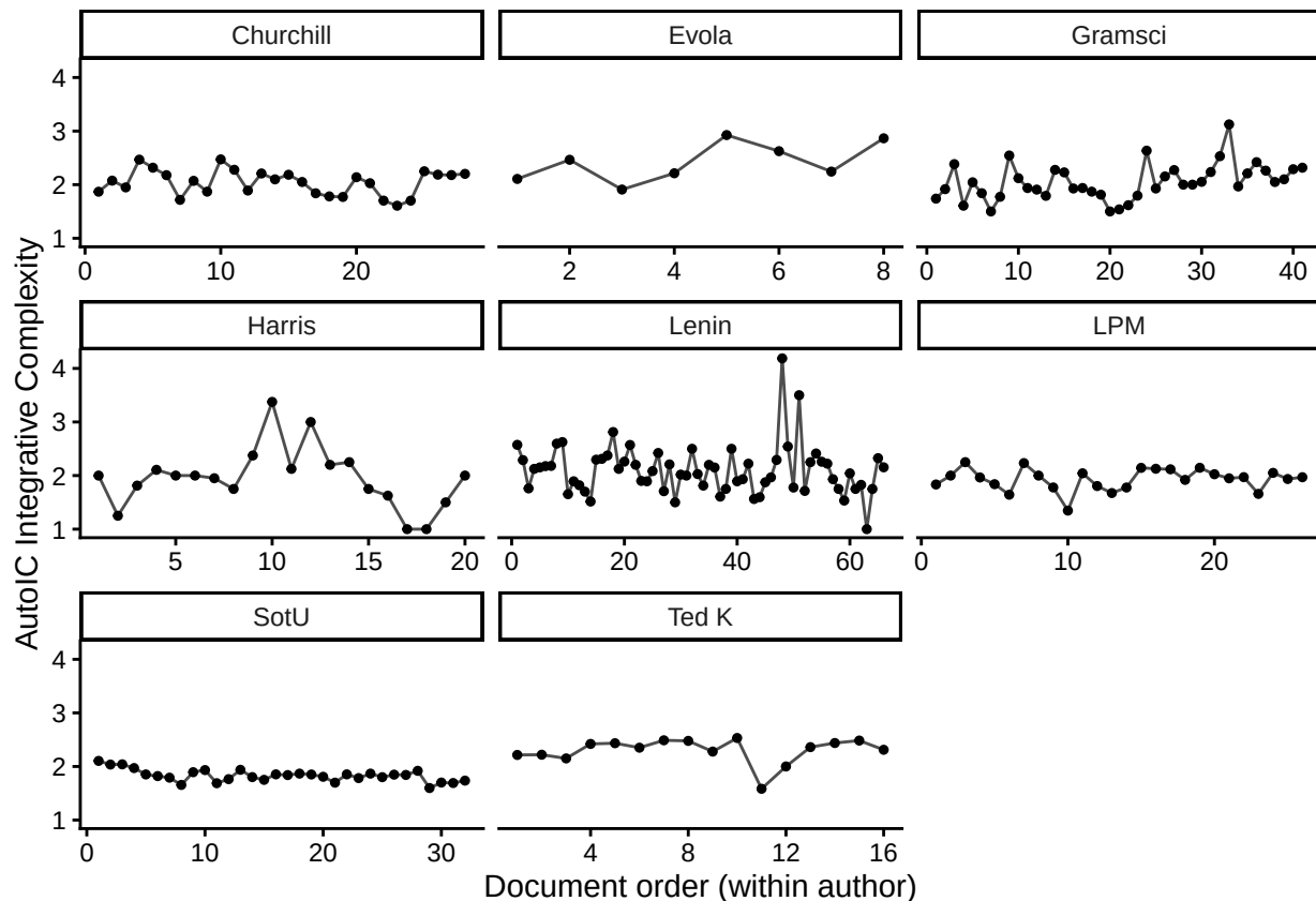
Figure 4. Longitudinal trajectories of integrative complexity by author (document order).
