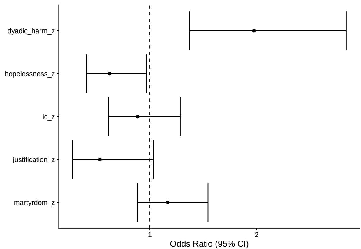
Figure 3. Odds ratios (95% CI) from the logistic model predicting violent (vs. non-violent) category.
