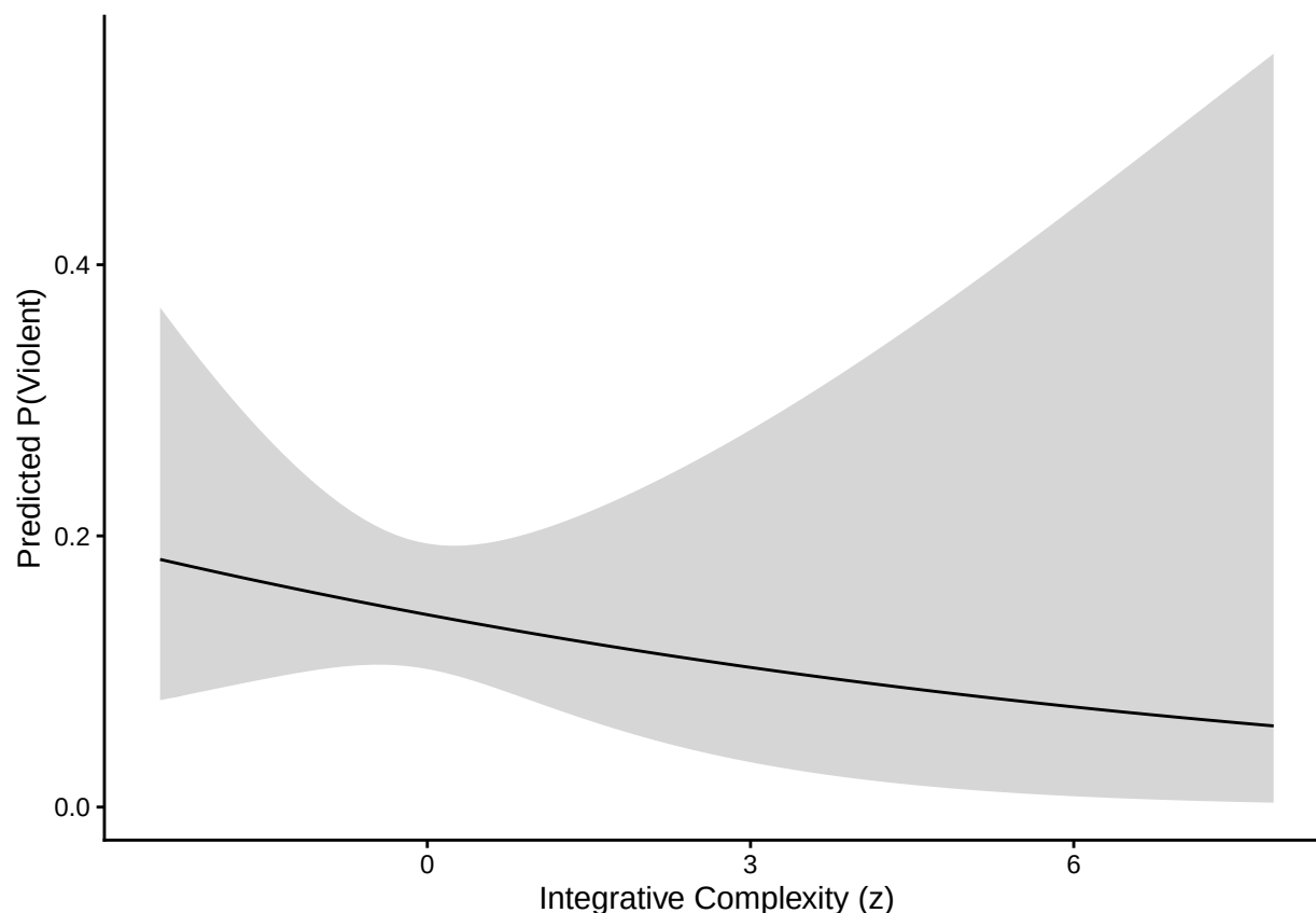
Figure 2. Predicted probability of violent (vs. non-violent) category as a function of integrative complexity (95% CI).
