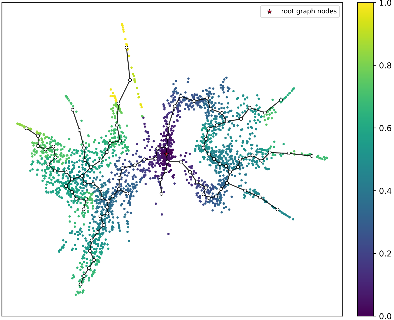
Classical MDS alpha=0 / ncenter120_nnk28_minbranch3
