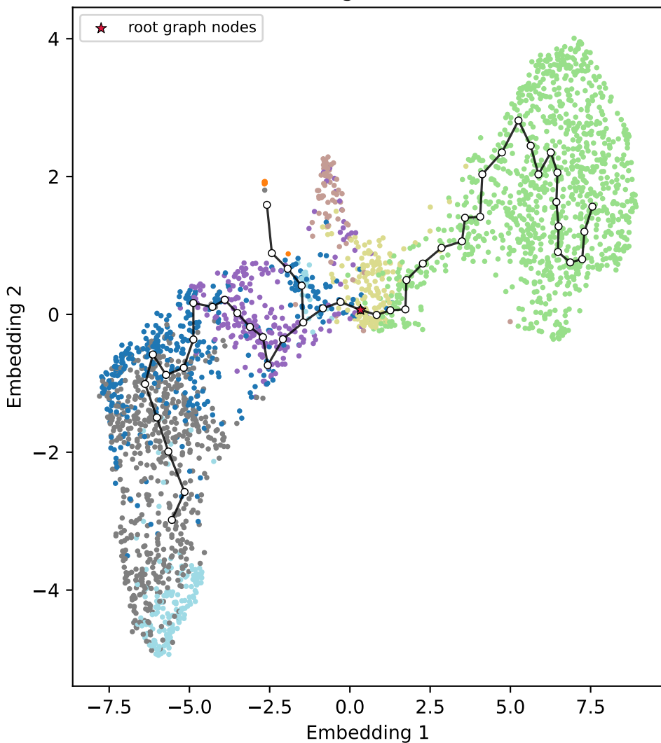
Paul15 MDS-geodesic clusters
