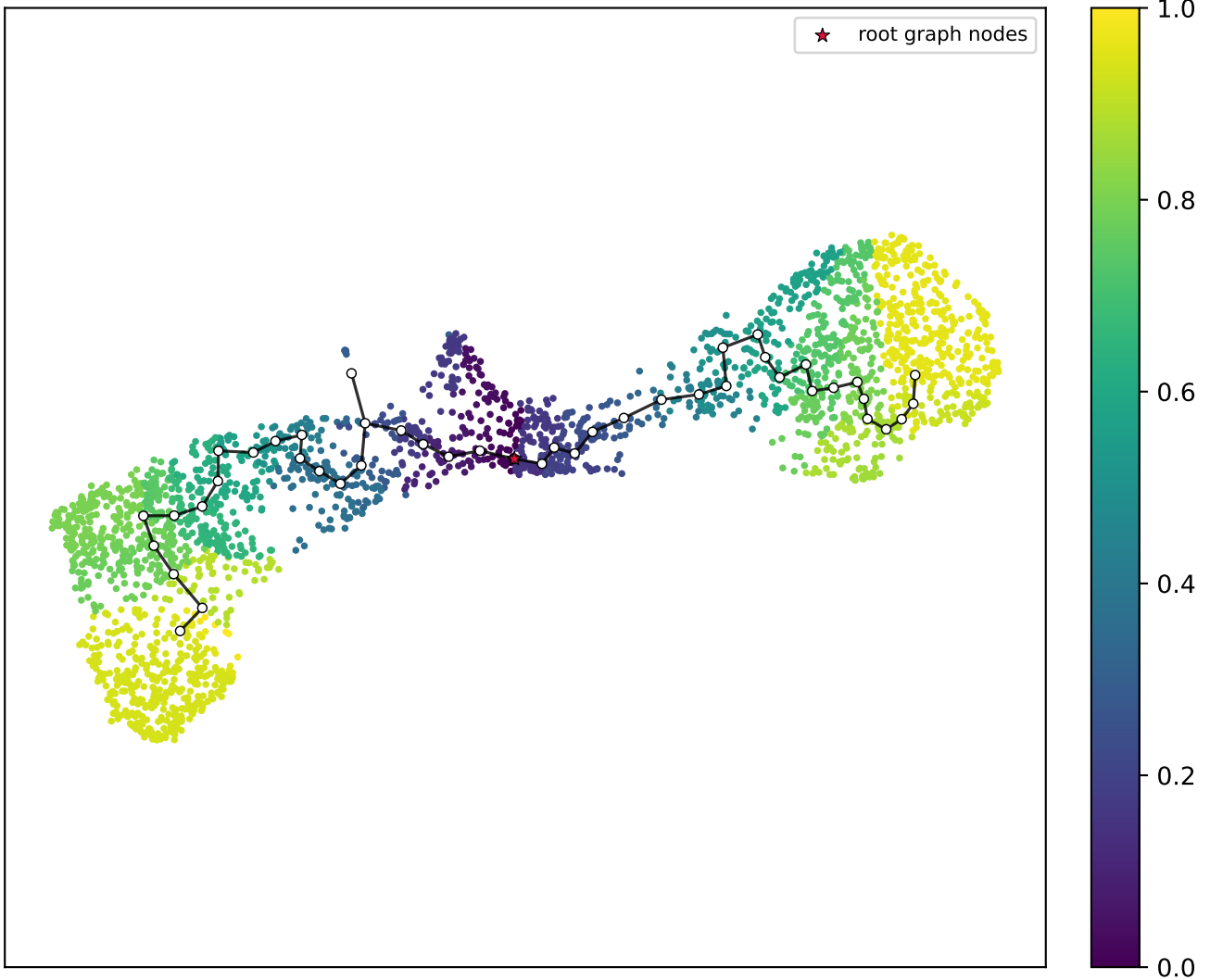
UMAP coordinates, Monocle-UMAP pseudotime + principal graph
