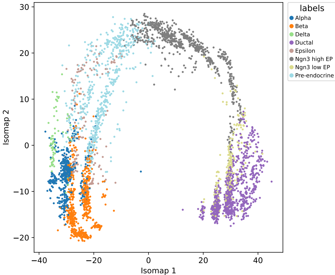
scVelo pancreas Isomap 2D
