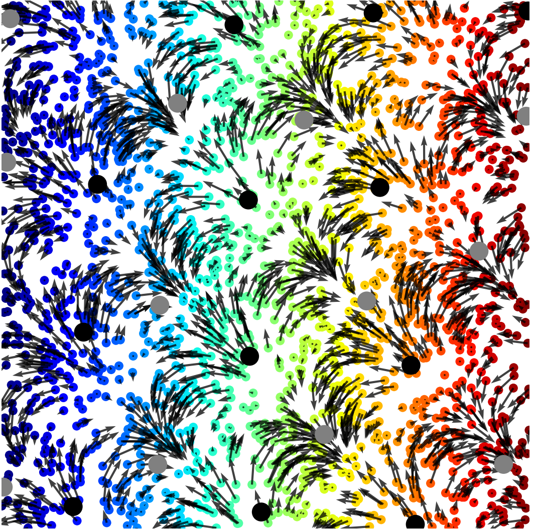
Sea1 vortical current map, \alpha=0.8
