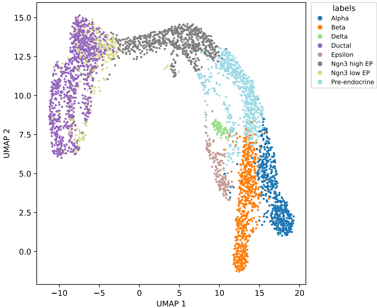
scVelo pancreas UMAP
