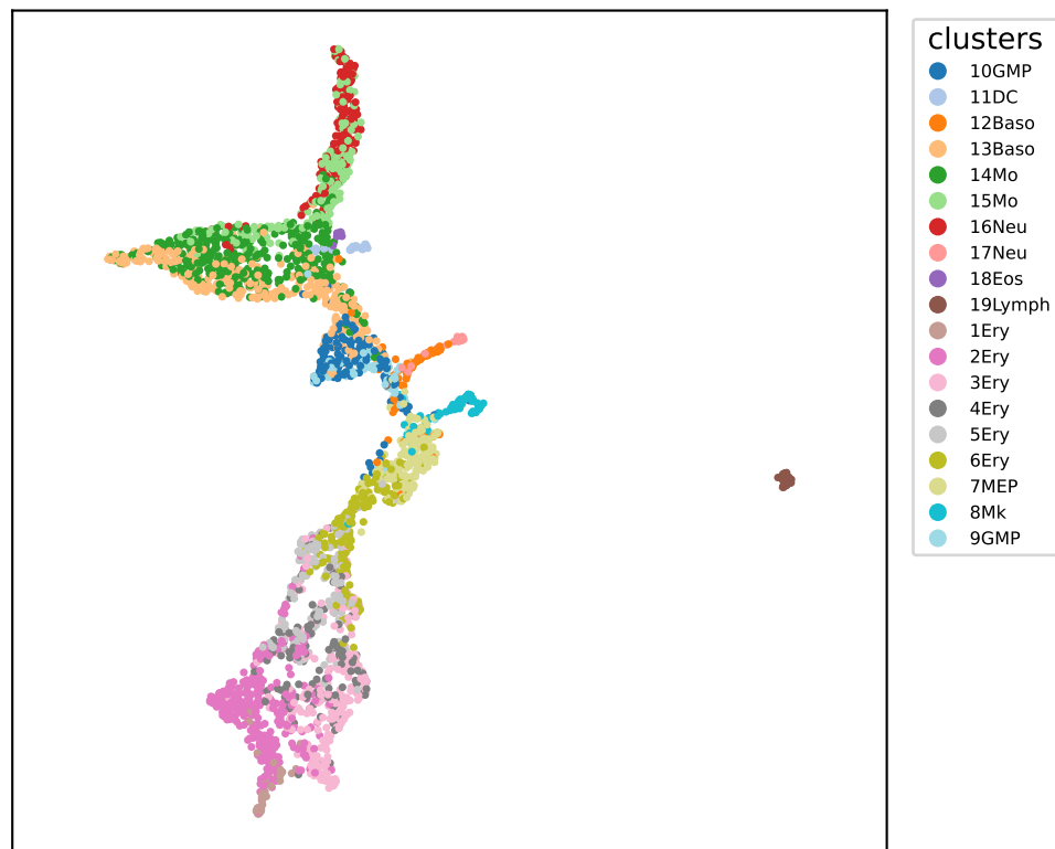
Paul15 clusters / UMAP
