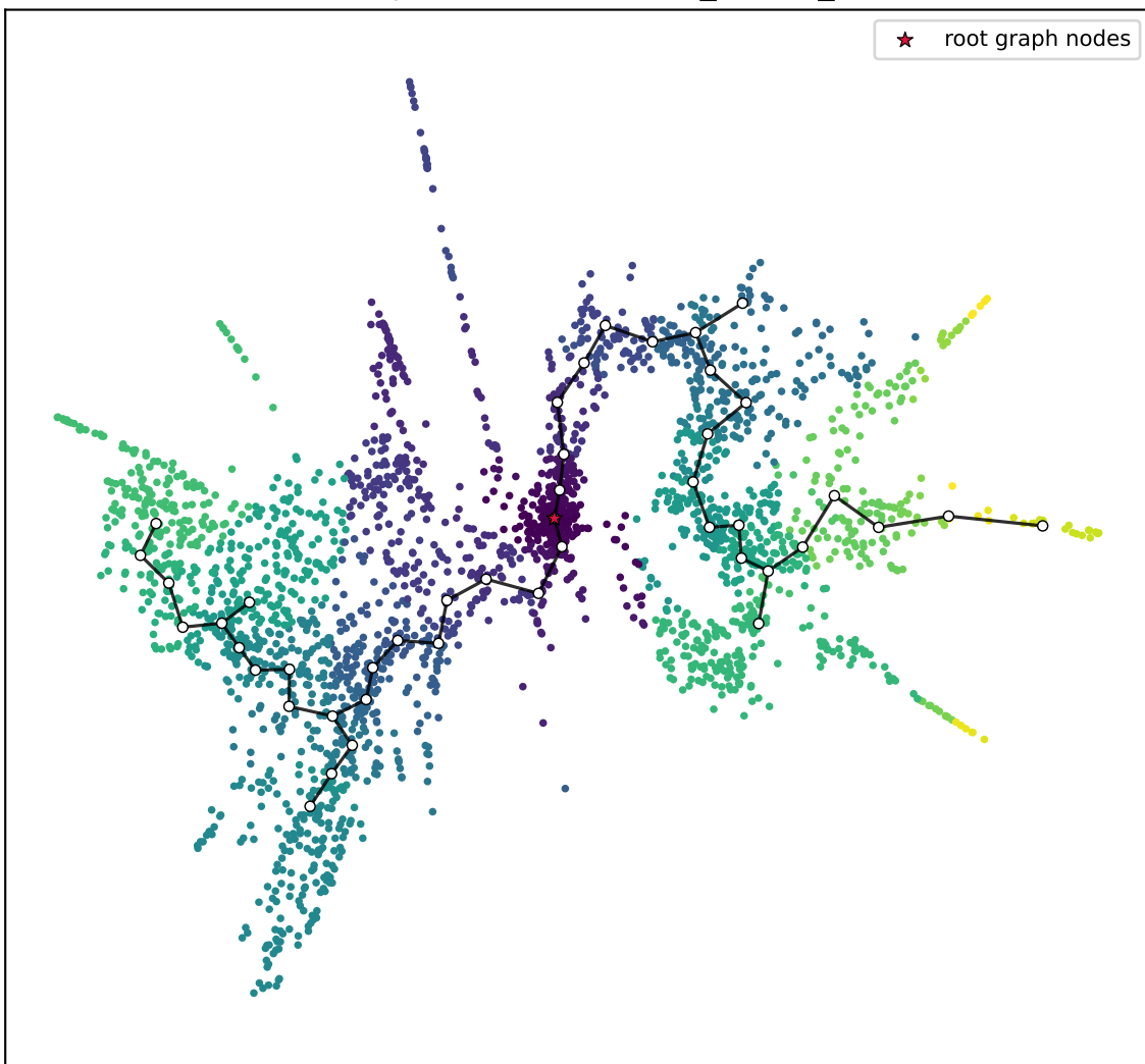
Classical MDS alpha=0 / ncenter85_nnk35_minbranch5
