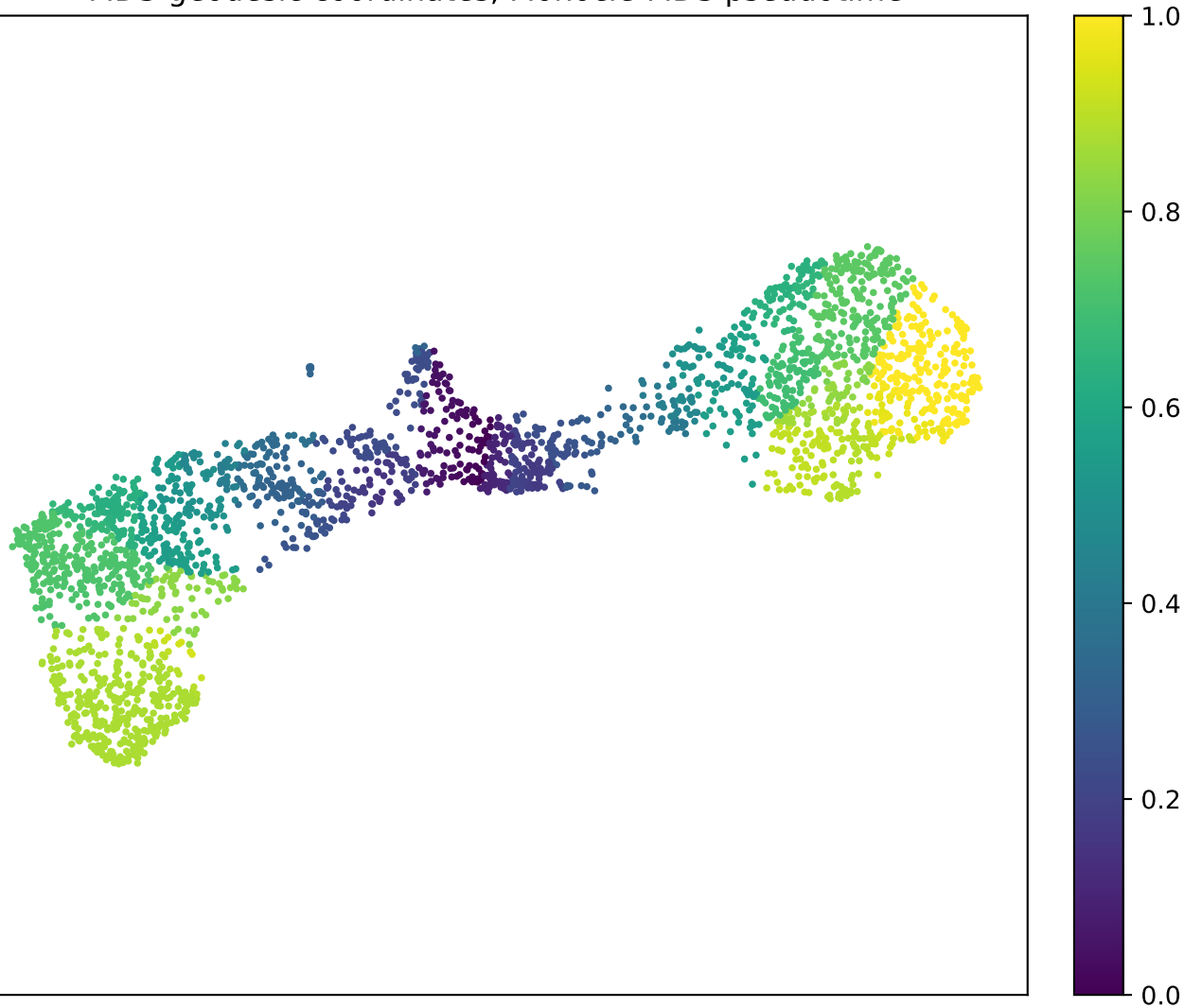
MDS-geodesic coordinates, Monocle-MDS pseudotime
