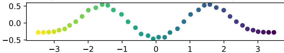
Toy two-bump: path-frozen Matsumoto \alpha=0.4
