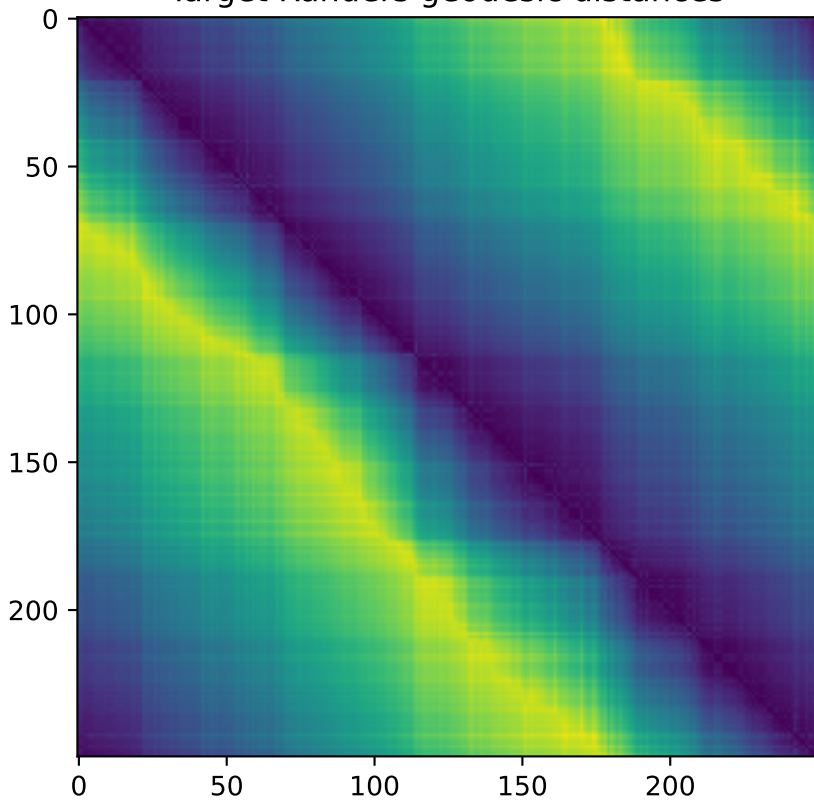
Target Randers geodesic distances
