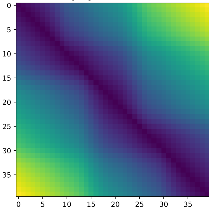
Target geodesic distances
