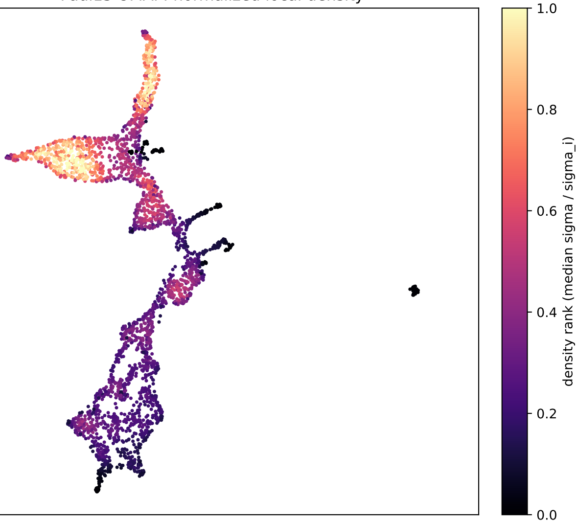
Paul15 UMAP: normalized local density
