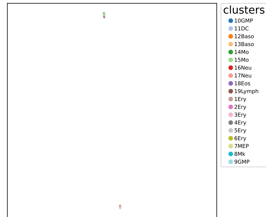
SMACOF
