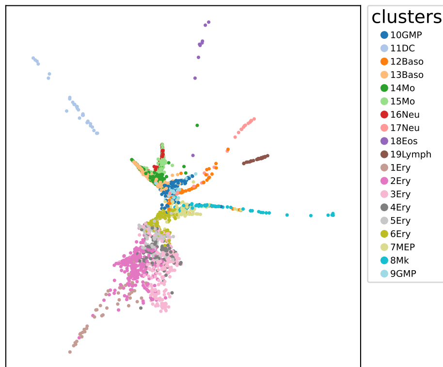
SMACOF
