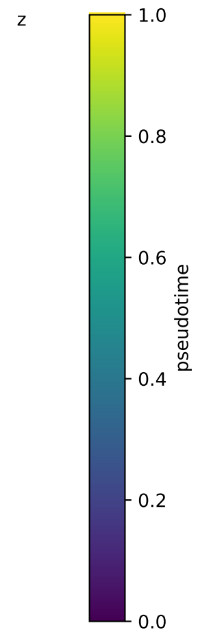
Path-frozen Randers alpha=0 (side)
